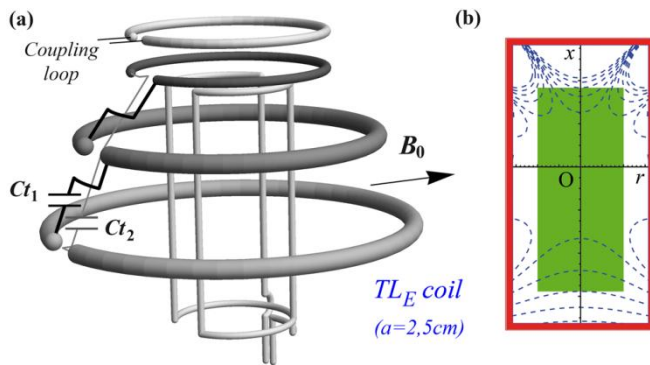
Fig. 8. (a) Schematic diagram of the rf gradient coil prototype (type TL_E ) with balanced tuning capacitors Ct_1 and Ct_2 , and a tuned matching coupling loop. A saddle-shaped coil (diameter: 1.65cm, height: 3.3cm) is used for normal transmit-receive NMR operations. (b) Overview of the deviation of the gradient field in an axial section of the saddle-shaped coil: iso-gradient contours are extracted from Fig. 6. The deviation from the maximum gradient value is less than 10% in a cylindrical volume with 1 cm in diameter and 2.4 cm in height (represented by a green filled rectangle).
