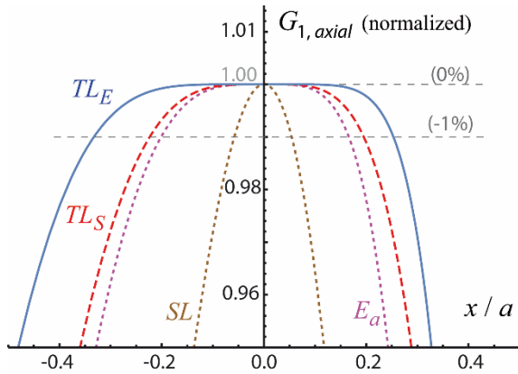
Fig. 3. Computed normalized rf field gradient G_{1,axial} : profiles along the symmetry axis for the three-coil systems TL_E (solid line in blue) and TL_S (dashed line in red), for an optimized two-loop system [12] E_a (dotted line in purple) and for a single loop SL (dotted line in brown). For the four systems, a is the radius of the outer coil.
