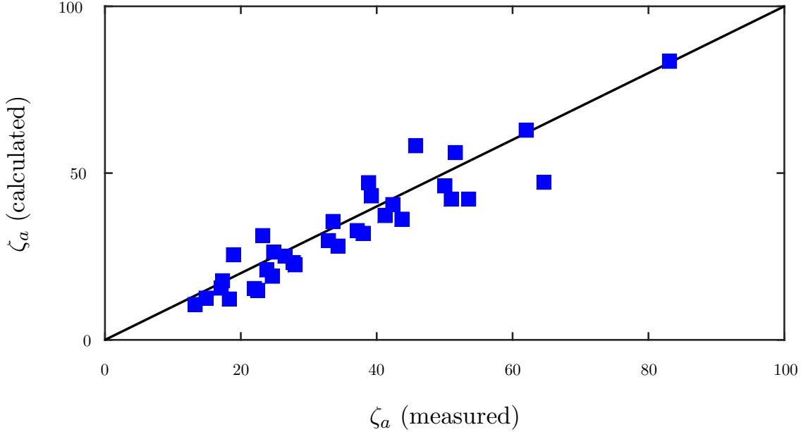
FIG. 9: Comparison between the experimental data and the numerical solution of (23).
