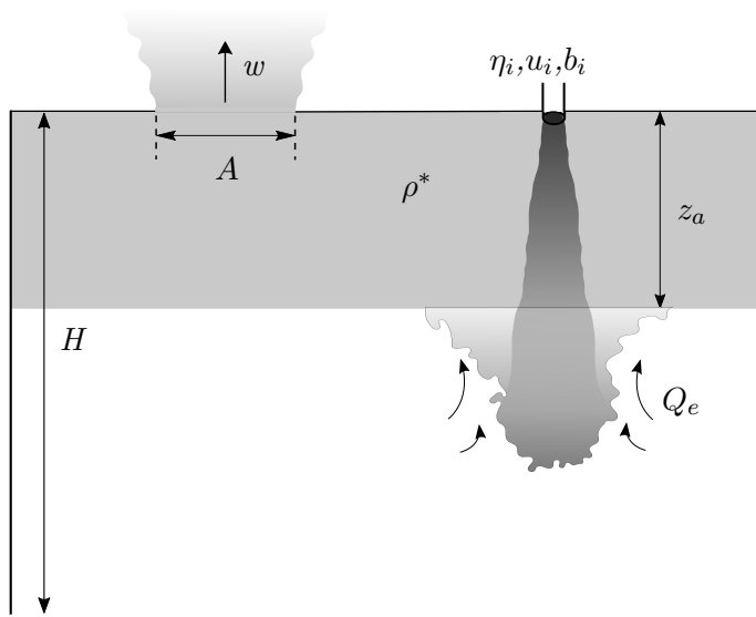
FIG. 5: Schematic of the fountain filling a box and simultaneously emptied by an opening vent on the ceiling. Note that A corresponds to the vent area.
