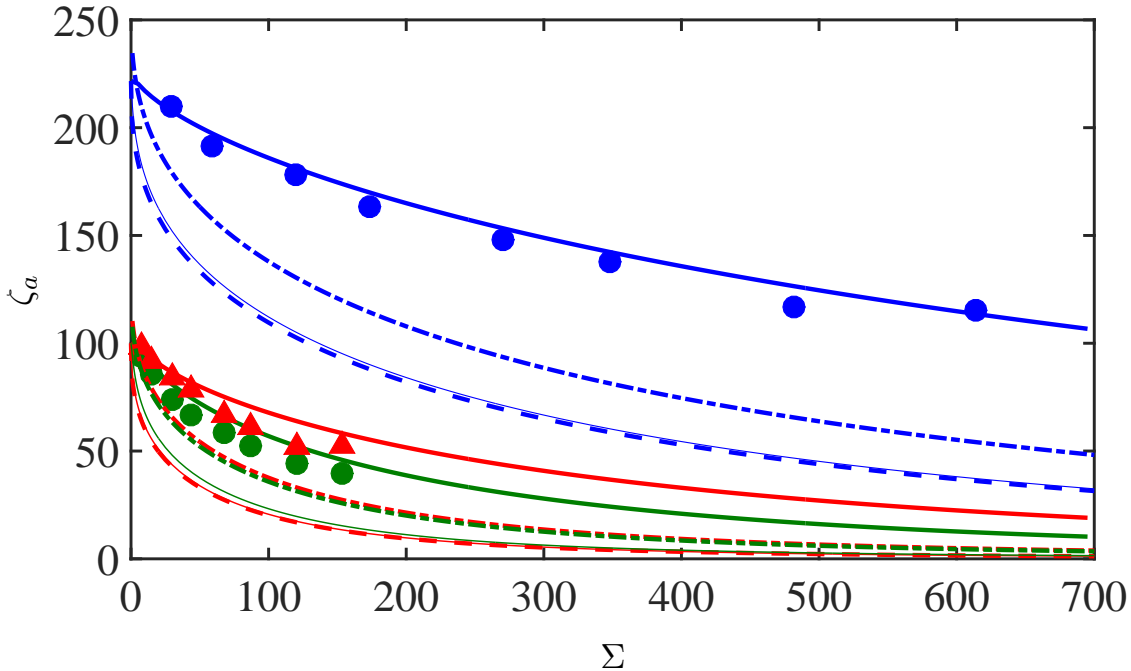
FIG. 4: The dimensionless thickness of the buoyant layer ( \zeta_a ) as a function of the parameter \Sigma , for three different configurations. The solid thick lines correspond to the numerical solutions of Eqs[12, 13], the thin solid lines corresponds to the numerical solutions of equation (14), the dashed thick lines corresponds to equation (15) and the thick dashed-dotted line corresponds to equation (16). The symbols correspond to the experimental data: (●) configuration 1, (▲) configuration 2 and (■) configuration 3 .
