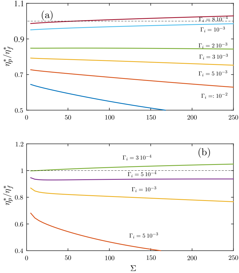
FIG. 12: Ratio \eta_p^*/\eta_f^* as a function of \Sigma for different values of \Gamma_i : (a) corresponds to a source density deficit of \eta_i = 0.05 , (b) corresponds to \eta_i = 0.85 and for both figures H/b_i = 200 . The dashed lines correspond to \eta_p^*/\eta_f^* = 1 .
