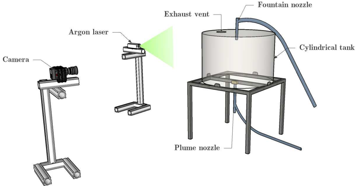
FIG. 1: Schematic of the experimental apparatus.
