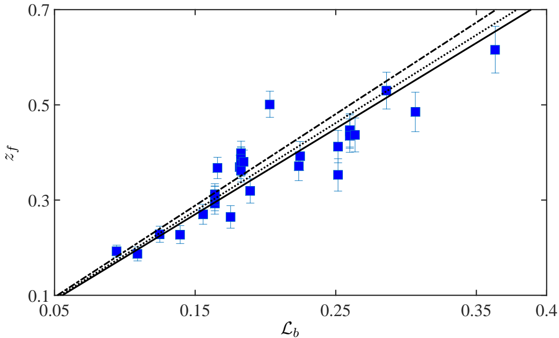
FIG. 6: Plot of the fountain height as a function of the length scale \mathcal{L}_b : the blue squares correspond to the experimental points, the solid black line corresponds to z_f \approx 1.8 \mathcal{L}_b , the dotted line corresponds to z_f \approx 1.84 \mathcal{L}_b given by [6, 34] and the dashed line corresponds to z_f \approx 1.92 \mathcal{L}_b given by [20]. The bars correspond to the amplitude of oscillation of the fountain height set to 0.14 \mathcal{L}_b as suggested by [20].
