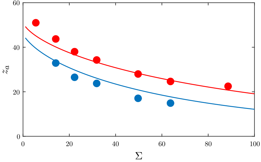
FIG. 8: Variation of z_a as a function \Sigma for two different values of \Gamma_i : the blue color corresponds to \Gamma_i = 0.0087 and the red color corresponds to \Gamma_i = 0.0114 .
