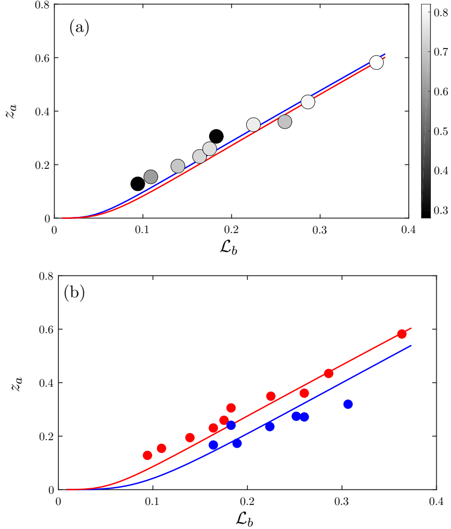
FIG. 7: (a) Variation of z_a as a function of \mathcal{L}_b for a fixed value of \Sigma = 14.1 . The experimental data are shaded according to the density deficit \eta_i , the blue solid line corresponds to the numerical solution of (23) with \eta_i = 0.2 and the red line corresponds to \eta_i = 0.9 . (b) Variation of z_a as a function of \mathcal{L}_b for two different values of \Sigma , the coloured circles correspond to experimental data and the solid lines correspond to the theoretical predictions. The red color corresponds to \Sigma = 14.1 and the blue color corresponds to \Sigma = 31.8 .
