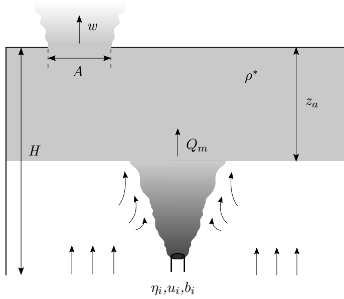
FIG. 3: Schematic of the plume fountain filling a box and simultaneously emptied by an opening vent on the ceiling. Note that A corresponds to the vent area.
