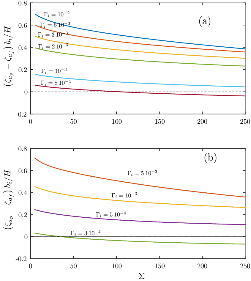
FIG. 10: Difference (\zeta_{a_p} - \zeta_{a_f}) b_i/H as a function of \Sigma for different values of \Gamma_i : (a) corresponds to \eta_i = 0.05 , (b) corresponds to \eta_i = 0.85 and for both figures H/b_i = 200 .
