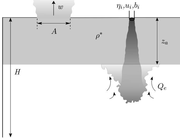
FIG. 5: Schematic of the fountain filling a box and simultaneously emptied by an opening vent on the ceiling. Note that A corresponds to the vent area.
