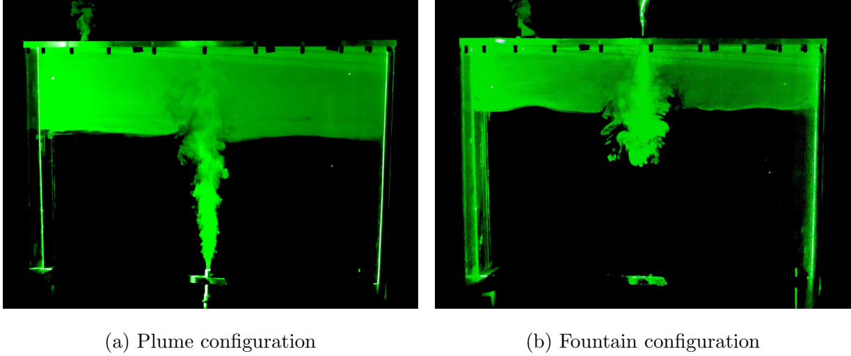
FIG. 2: Illustration of plume and fountain filling-emptying box experiments.
