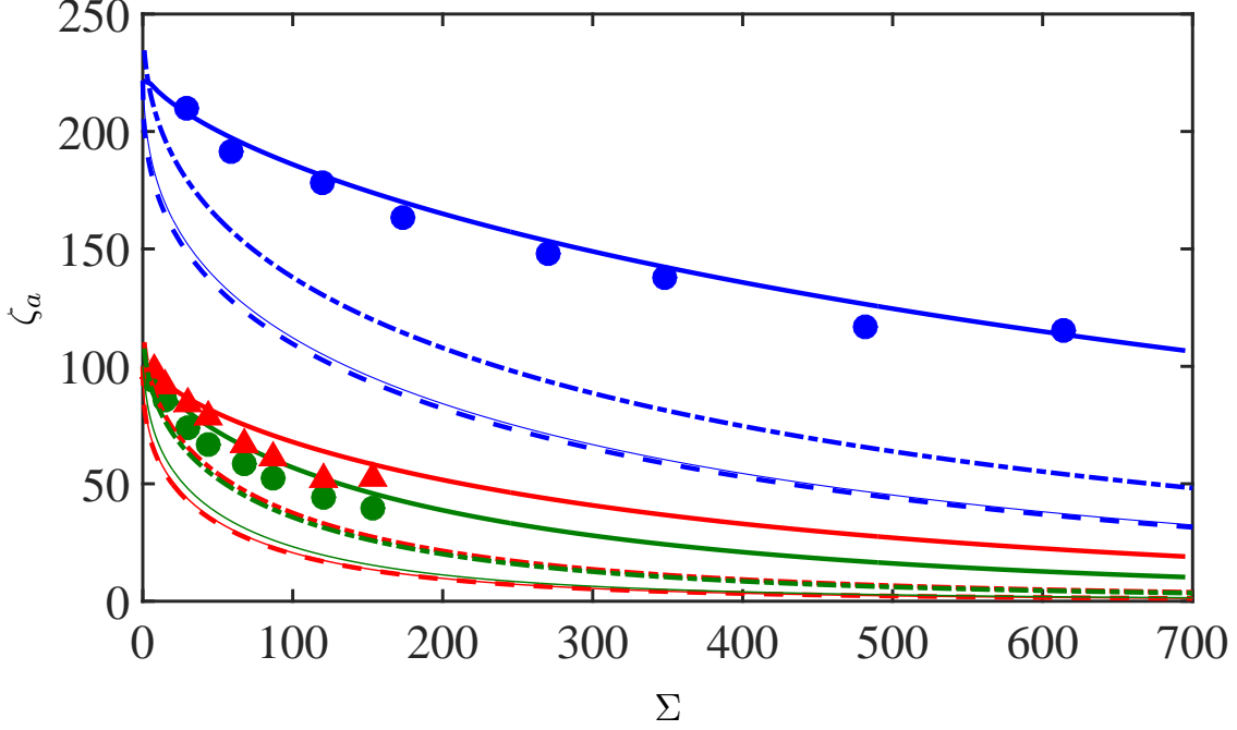
FIG. 4: The dimensionless thickness of the buoyant layer ( \zeta_a ) as a function of the parameter \Sigma , for three different configurations. The solid thick lines correspond to the numerical solutions of Eqs[12, 13], the thin solid lines corresponds to the numerical solutions of equation (14), the dashed thick lines corresponds to equation (15) and the thick dashed-dotted line corresponds to equation (16). The symbols correspond to the experimental data: ( \bullet ) configuration 1, ( \blacktriangle ) configuration 2 and ( \blacksquare ) configuration 3 .
