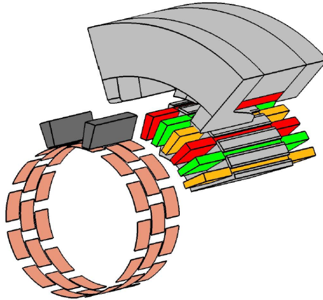
Figure 10. FE-model of claw pole structure with its commutator
