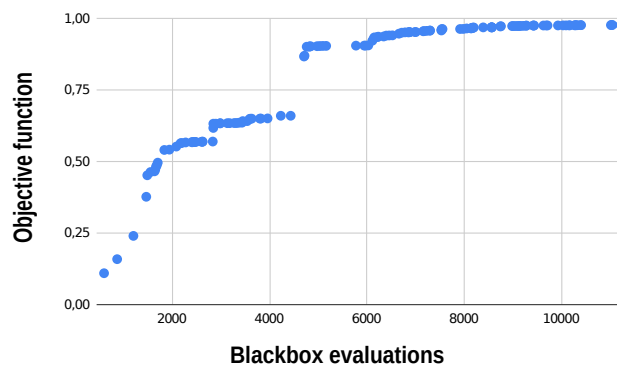
Figure 11. Convergence of objective function vs. number of blackbox evaluations
