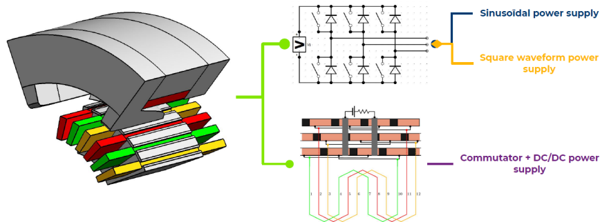
Figure 6. Different supply solution for claw pole machine
