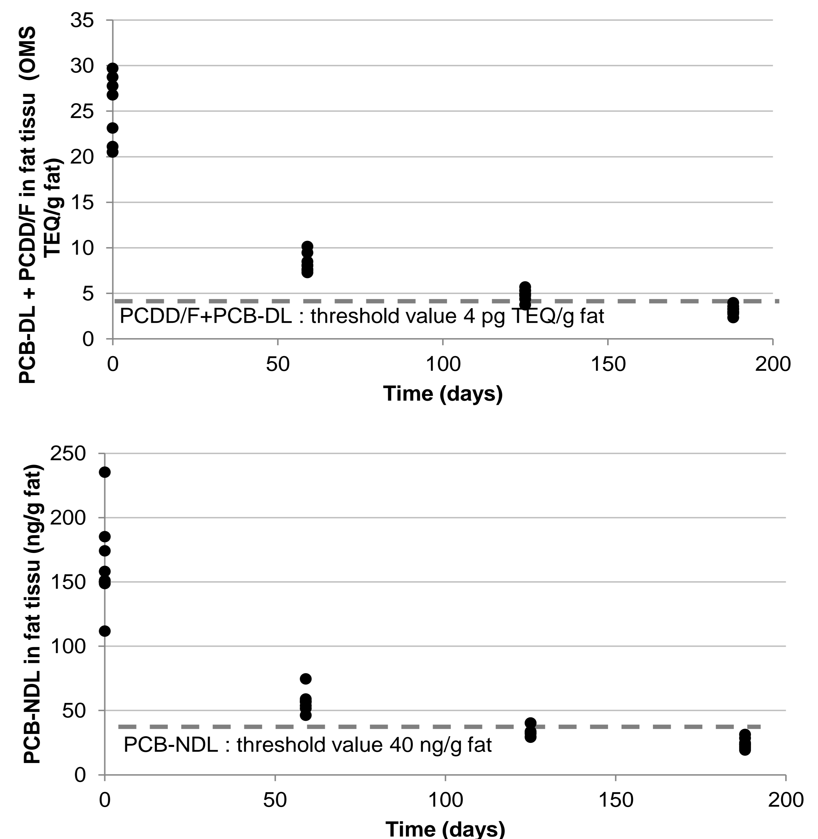
Figure 1 : Decontamination kinetics of DL PCB and NDL PCB in growing limousine heifers
