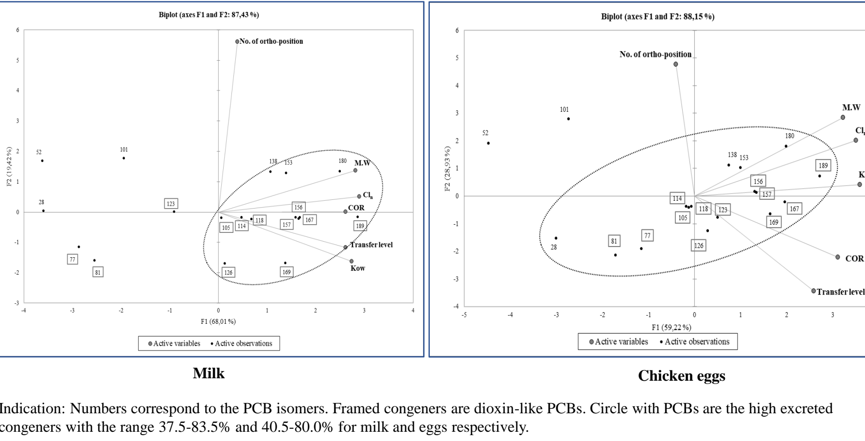
Factorial plan (F1, F2) of PCA applied on mean CORs of PCBs for milk (A) and eggs (B), chlorine substitution at none, mono and di-ortho position, number of chlorines, molecular weight (M.W.), n-Octanol/Water Partition Coefficient (K ow ) and transfer level.
