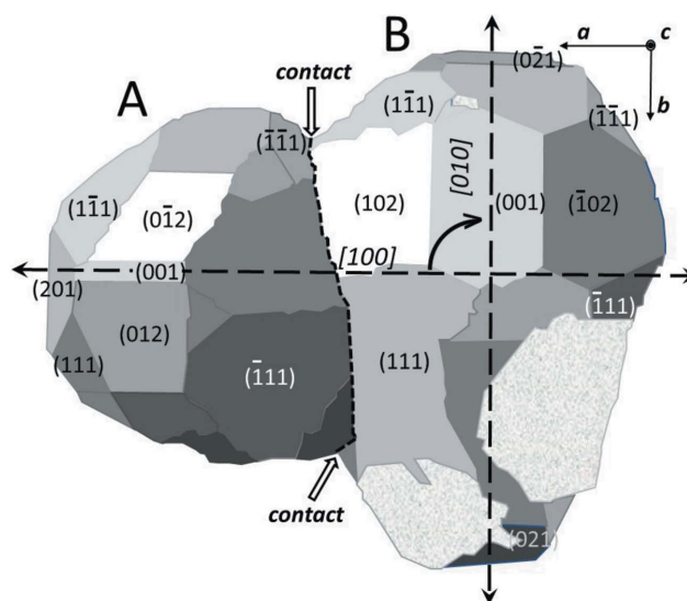
Figure 14 Scheme along c of V contact twin, with indication of the twin law according to a 90° rotation around c axis. Curved arrow: 90° rotation from [100] to [010] directions (double-headed arrows).
