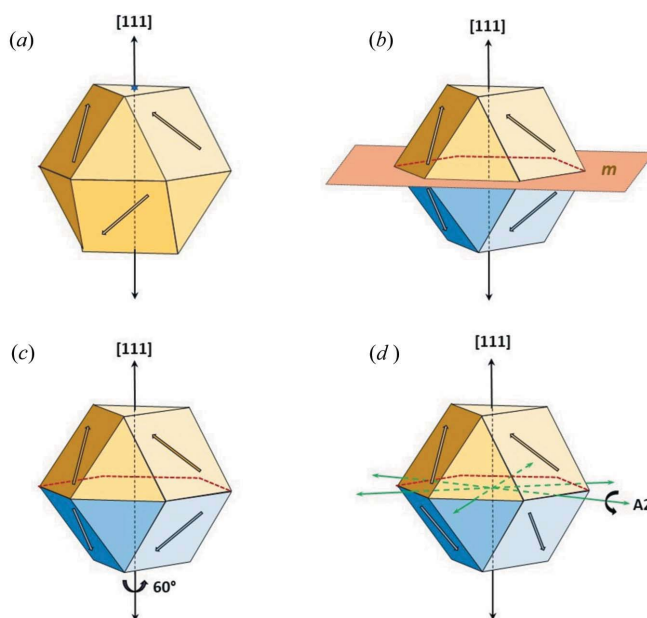
Figure 17 Comparison of the spinel twin and the Gaubert twin, starting from a pyrite cuboctahedron (a). The spinel twin with indication of the mirror m , or the (2 n +1)60° rotation around the [111] axis: (b) and (c), respectively. (d) The Gaubert twin according to an 180° rotation about a direction contained in the (111) plane ([211], [121] or [112] – double-headed green arrows).
