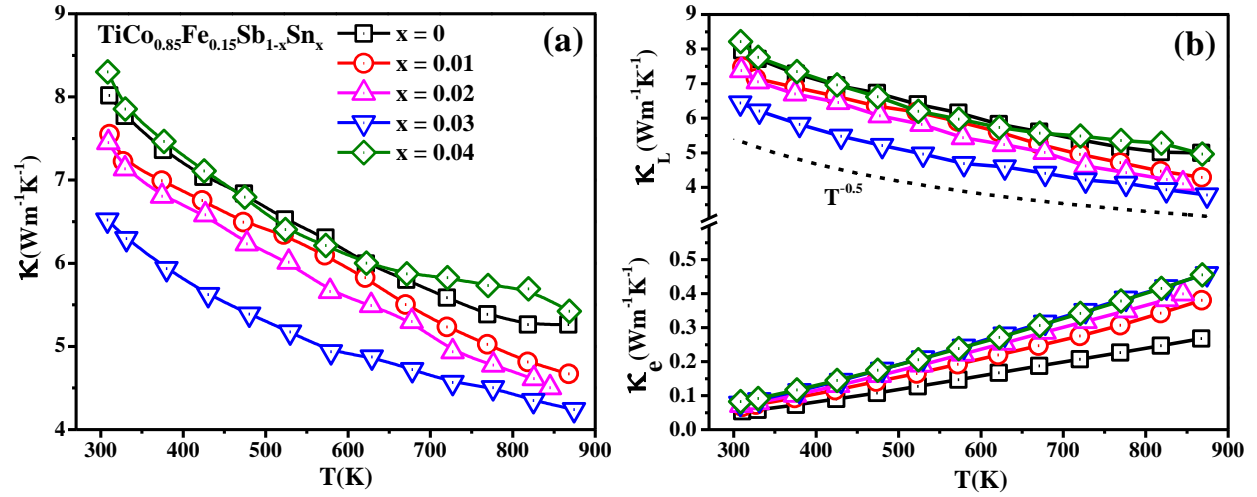
Fig. 7: (a) Total thermal conductivity and (b) electronic and lattice thermal conductivity as a function of temperature of the \text{TiCo}_{0.85}\text{Fe}_{0.15}\text{Sb}_{1-x}\text{Sn}_x samples.
