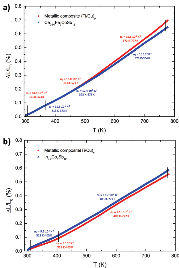
Figure 2. Thermal expansion \Delta L/L_0 of the a) p-type and b) n-type skutterudites as a function of temperature. The temperature dependence of the thermal expansion of the (\text{Ti}/\text{Cu})_n and (\text{Ti}/\text{Cu})_p metallic composites are also shown for comparison. For each material, the thermal expansion coefficients \alpha_T = \frac{1}{L_0} \left( \frac{\partial \Delta L}{\partial T} \right) is indicated in the different temperature ranges highlighted by the vertical black lines.
