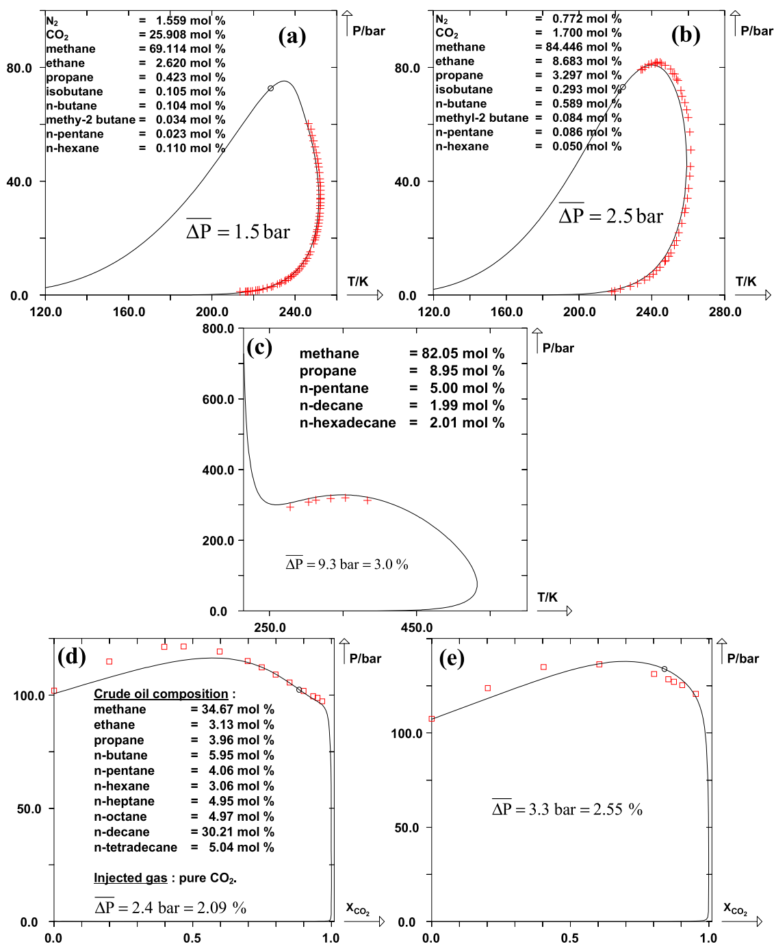
Fig. 3. Predictions of the phase behaviour of petroleum fluids by the PPR78 model ((+, \square ) experimental points, (O) calculated critical points, and lines: calculated saturation curves). (a) and (b): Phase envelopes of natural gases. (c) Phase envelope of a gas condensate. (d) and (e) Modelling of the swelling experiments of a petroleum fluid with pure CO 2 at 322 K and 338.7 K, respectively. \overline{\Delta P} denotes the mean deviation between the calculated and experimental pressures.
