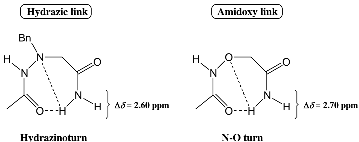
Figure 1. Comparison of \Delta\delta values between hydrazidic and amidoxy links by 1 H NMR (300 MHz, CDCl 3 /10 mM).
