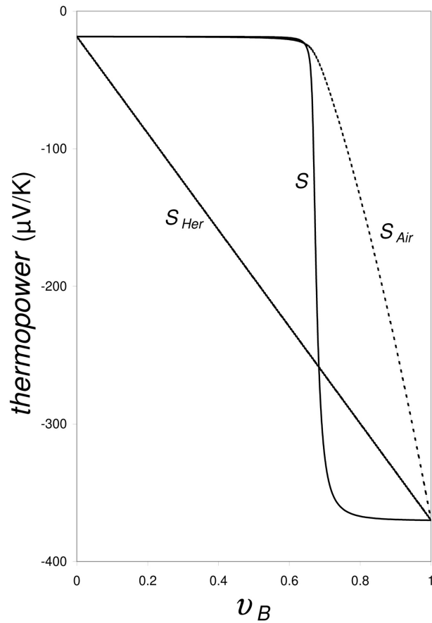
Figure 1. Comparison of S_{Air} , S_{Her} , and S vs. v_B calculated by Equation (46), Equation (56), and Equation (31), respectively, where S_A = -18.5 \mu\text{V/K} , \sigma_A = 7450 \Omega^{-1} \cdot \text{cm}^{-1} , \kappa_A = 0.022 \text{ W} \cdot \text{K}^{-1} \cdot \text{cm}^{-1} , S_B = -370 \mu\text{V/K} , \sigma_B = 7 \Omega^{-1} \cdot \text{cm}^{-1} , \kappa_B = 0.070 \text{ W} \cdot \text{K}^{-1} \cdot \text{cm}^{-1} [the numbers for S_i , \sigma_i , and \kappa_i are taken from [17] (Figure 2 therein); the quotients of them, S_B/S_A , \sigma_B/\sigma_A , and \kappa_B/\kappa_A correspond nearly to those applied in [webman] (Figure 2 therein).
