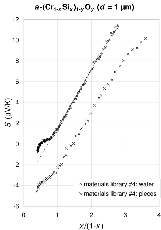
Figure 9. S vs. x/(1-x) of a \text{Cr}_{1-x}\text{Si}_x\text{O} thin film with an additional O gradient vertical to the wafer surface as well as in the same direction as those of silicon concentration gradient (measured for the complete wafer and the pieces after sawing to 8 \times 2 \text{ mm}^2 pieces). The measuring positions with respect to the wafer, before and after sawing, were the same ones. This figure is taken from [62].
