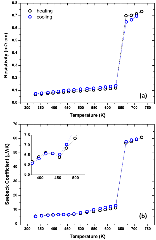
Figure 7. a) Electrical resistivity and b) Seebeck coefficient of \text{Cu}_{2.9}\text{Te}_2 as a function of temperature showing metallic behavior with a strong transition at 650 K and comparatively minor change at 450 K (see inset figure in (b)).
