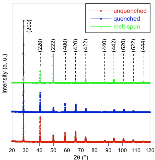
Figure 1. XRD patterns obtained on ground unquenched and quenched ingots and ground melt-spun ribbons. The main reflections are indexed.
