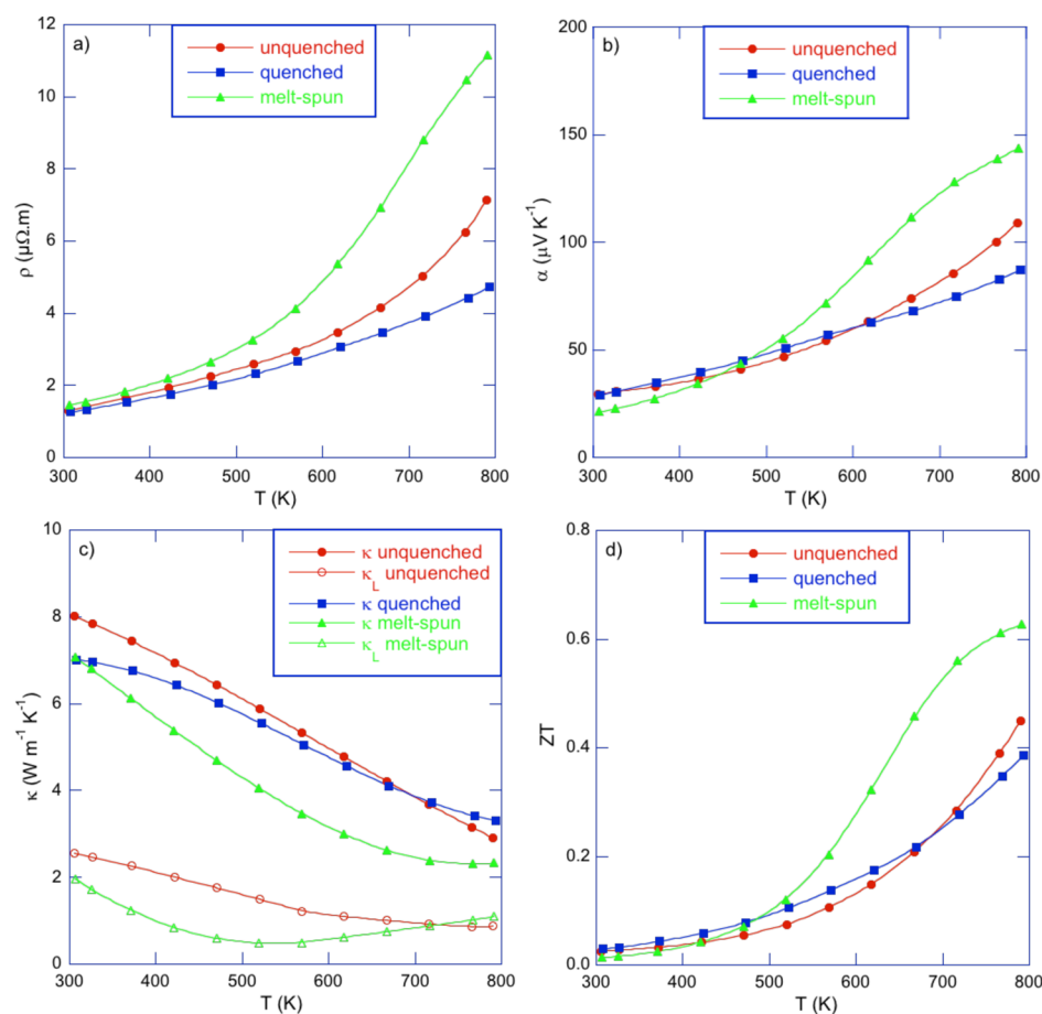
Figure 4. Temperature dependences of the (a) electrical resistivity \rho and (b) thermopower \alpha of the unquenched, quenched, and melt-spun samples. (c) Total (filled symbols) and lattice (open symbols) thermal conductivities as a function of temperature for the three samples. (d) Temperature dependence of the dimensionless figure of merit ZT for the unquenched, quenched, and melt-spun samples. In all panels, the solid lines are guides to the eye.
