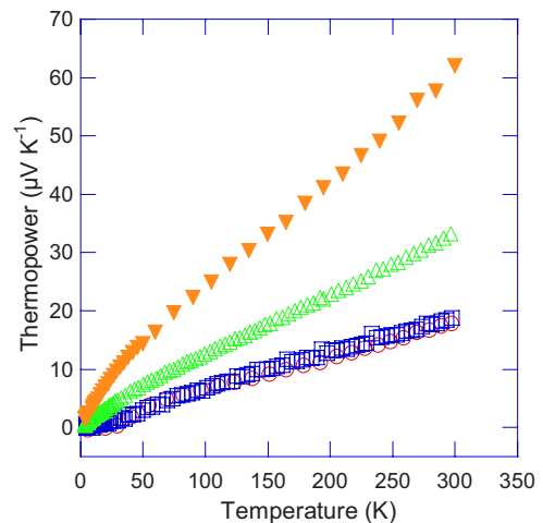
FIG. 10. (Color online) Temperature dependence of the thermopower for the x=0 (○), 0.25 (□), 0.5 (△), and 0.8 (▼) samples.
