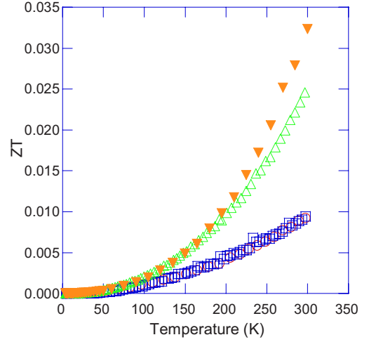
FIG. 13. (Color online) Temperature dependence of the thermoelectric figure of merit for the x=0 ( \circ ), 0.25 ( \square ), 0.5 ( \triangle ), and 0.8 ( \blacktriangledown ) samples.
