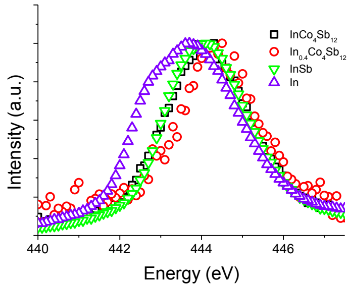
Fig. 4 XPS spectra of \text{In}_{3d} energy level in \text{In}_{0.4}\text{Co}_4\text{Sb}_{12} , \text{InCo}_4\text{Sb}_{12} and reference materials In and InSb.
