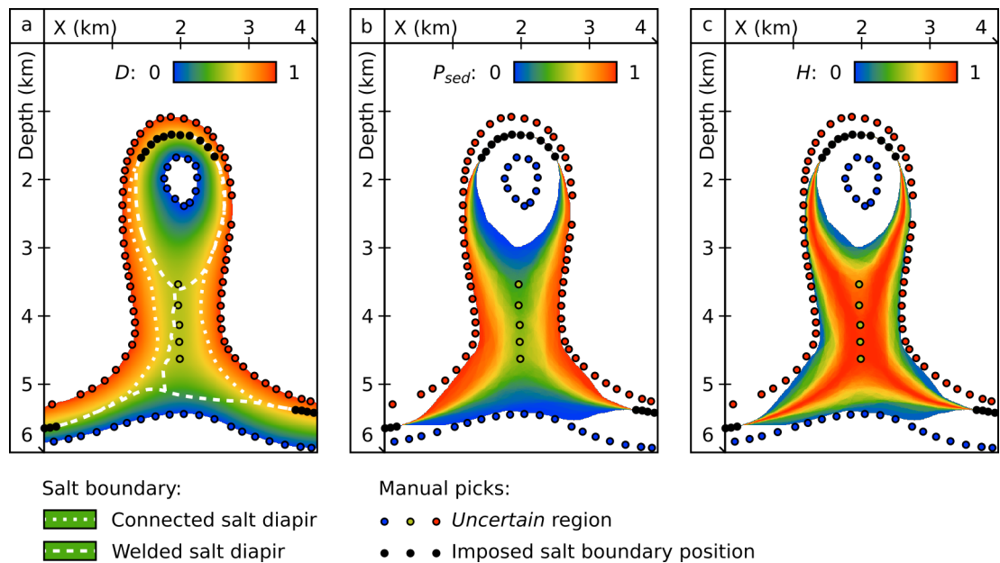
Figure 3 Variability of the simulated salt boundary interpretations. (a) Reference field D and the two interpretations which have been selected for seismic modeling (white dotted and dashed lines). (b) Posterior sediment probability P_{sed} (equation 2). (c) Information entropy H (equation 3). The white parts of the Uncertain region in (b) and (c) indicate that the facies at the pixel location is constant over the 100 realizations.
