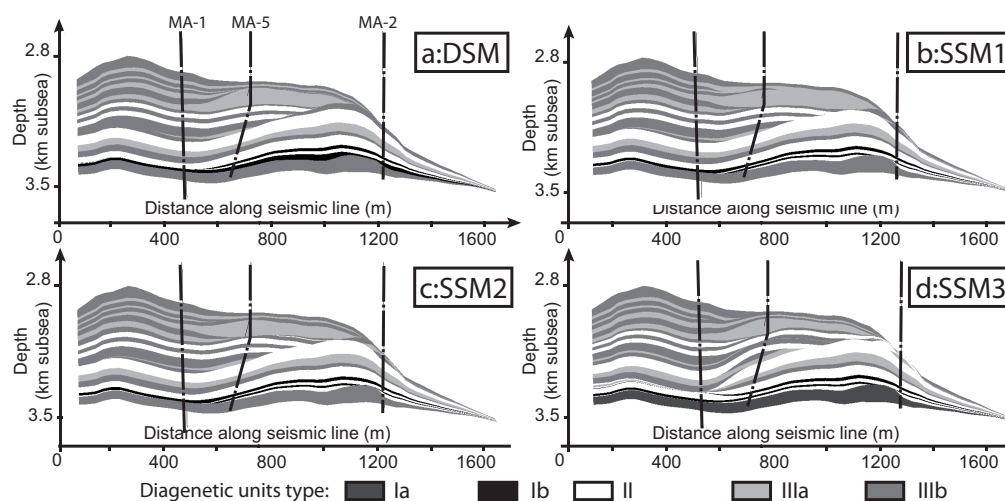
Figure 3: Sections of the diagenetic units model built from stratigraphic correlations computed using the proposed algorithm. The deterministic model is the minimum cost one. For reference, wells MA-1, 2 and 5 are projected on the section.
