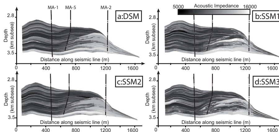
Figure 4: MA-1 to MA-2 cross-section of acoustic impedance models generated on grids built from DSM (a), SSM1(b), 2(c) and 3(d) using Sequential Gaussian Simulation.
