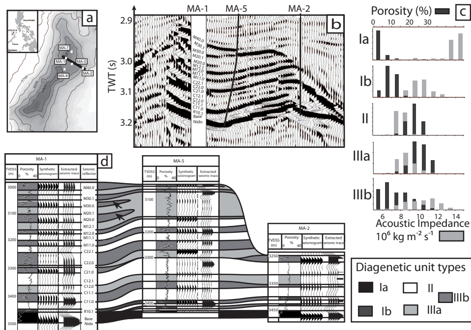
Figure 1: (a) Topographic map (in meter sub-sea) of the top horizon of the Malampaya gas reservoir located offshore western Palawan island, Philippines. (b) Seismic line between wells MA-1 and MA-2 displaying Malampaya interior reflector. (c) Porosity and acoustic impedance histogram for the different diagenetic unit types. (d) Stratigraphic model proposed by Fournier & Borgomano (2007) on the basis of wells and seismic interpretation. Modified after Grötsch & Mercadier (1999) and Fournier & Borgomano (2007).
