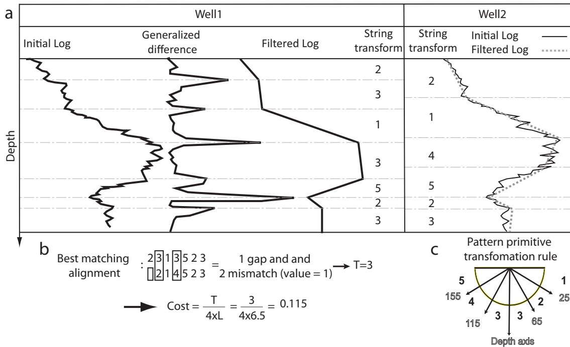
Figure 2: Evaluation of similarity between log responses of two units. Well logs are first filtered using generalized difference (a) and transformed into strings of pattern primitives according to dip angle of filtered log segments (c). Cost is computed as the difference between the two strings representing the two considered units (b). After Fang et al. (1992)
