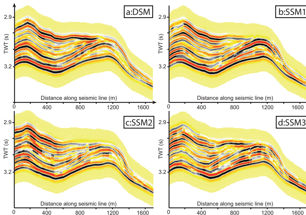
Figure 5: MA-1 to MA-2 cross-section of synthetic seismic amplitude model computed by convolution of acoustic impedance model (Fig.4) with a 50hz Ricker wavelet. All of the four seismic sections display comparable internal reflectors and may result in similar stratigraphic interpretation.
