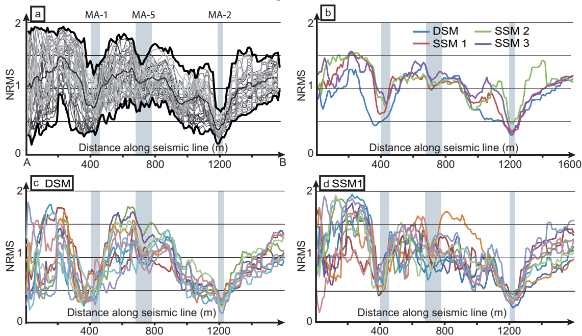
Figure 6: NRMS computed along the MA-1 to MA-2 section between one reference seismic amplitude model computed on DSM and forty alternative seismic models computed on DSM, SSM1, 2 and 3 (ten on each). On (a) are displayed all forty computed NRMS lines, maximum and minimum values (thick line) and mean values. (b) Mean values of NRMS for each stratigraphic correlation model show comparable values. The ten NRMS computed on DSM (c) and SSM1 (d) show comparable variations. NRMS dispersion observed at well location (grey zones) are due to well path deviation. The well MA-5 trajectory is projected on the studied cross section which explains the amplitude of dispersion at its location.
