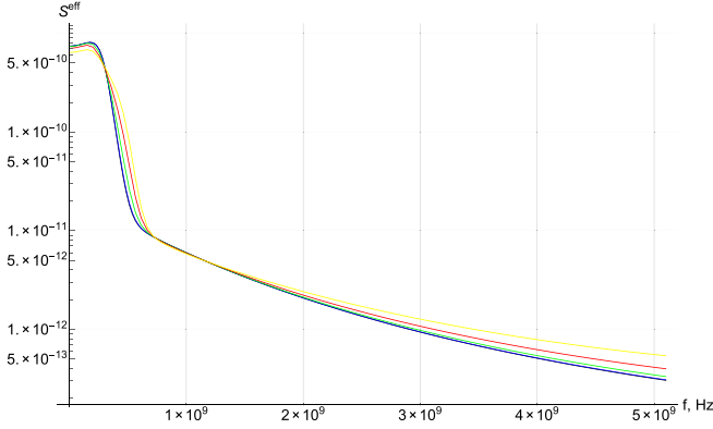
FIG. 3. Black curve (almost fully beyond the blue one) is S_{mn} ; the blue, green, red, and yellow curves stand for S_{mn}^{eff} for different turbulence amplitudes: 0%, 3%, 6%, and 10%, respectively. Without considering the local plasma inhomogeneity, \frac{k_0}{L} = 0 \text{ cm}^{-2} .
