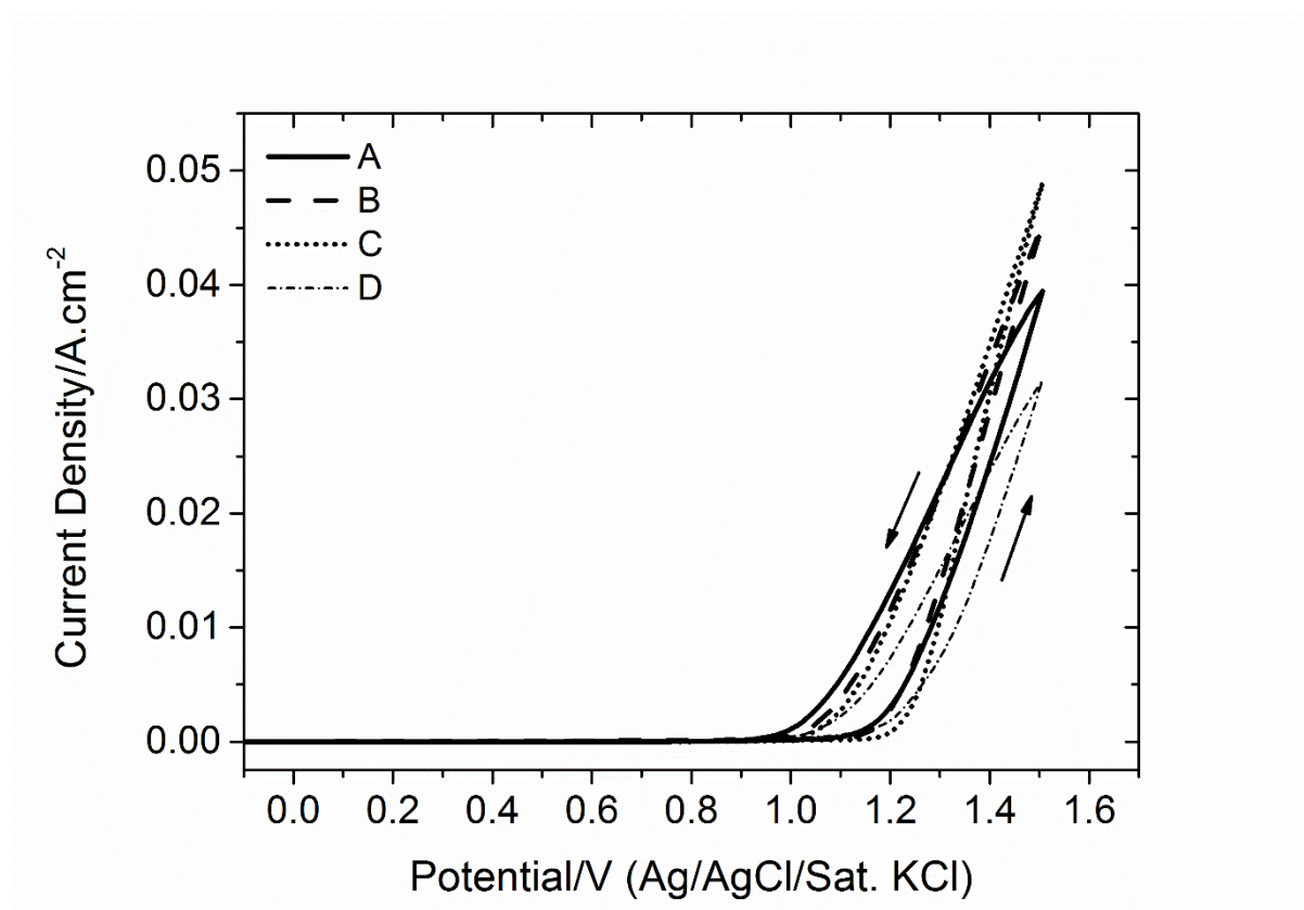
Fig. 1.a : Potentiodynamic current vs potential curves of Inconel 718 in solutions A, B, C and D. Scanning rate 10 mV s -1
