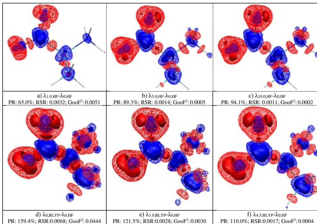
Figure 4. Plot of the difference in electron density for different \lambda values during the XCW fitting on L-alanine using CCSD structure factors of a resolution below 1.0778 \text{ \AA}^{-1} . Individual details are given in subcaptions. Isosurface values in a.u. (solid/wireframe): +0.005/+0.0025 (blue) and -0.005/-0.0025 (red). Representations for the other resolutions are given in the supplementary material.
