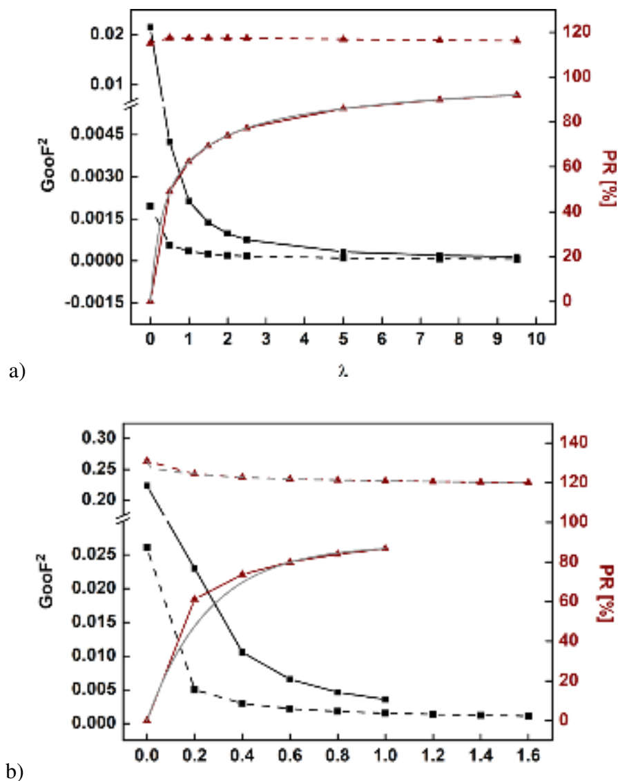
Figure 10. Graphs of structure factor and electron density agreement throughout XCWs at a resolution below 1.4415 \text{ \AA}^{-1} for urea (a) and 1.0778 \text{ \AA}^{-1} for L-alanine (b). GooF^2 (black) and the PR (red) plotted against the value of \lambda during the HF-XCW (solid) or HF-CC-XCW (dashed). Additionally exponential functions were fitted to the values to estimate the convergence limit of the PR (gray) according to eq. 5, except for HF-CC in a) as the function is too horizontal. CC = cluster charges.
