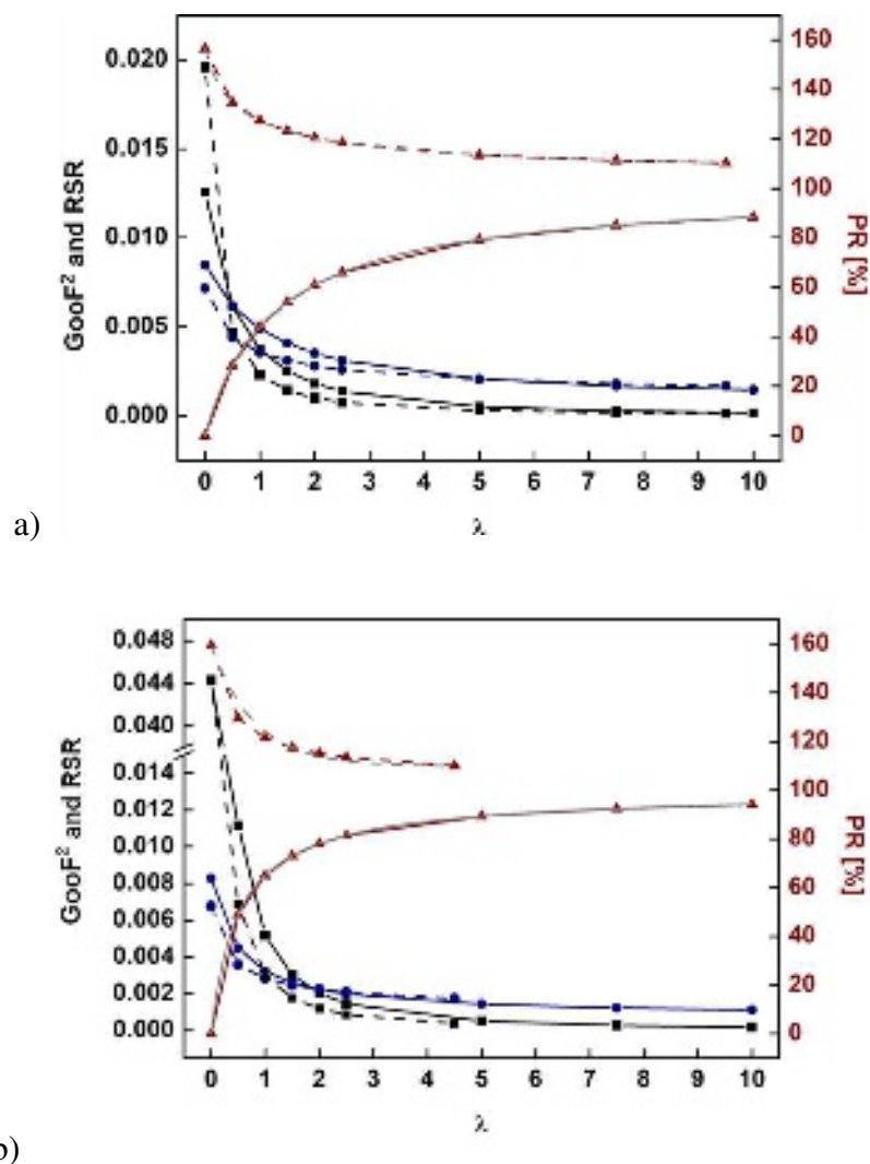
Figure 5. Graphs of structure factor and electron density agreement throughout XCW fittings a) for urea at a maximum resolution of 1.4415 \text{ \AA}^{-1} and (b) L-alanine at 1.0778 \text{ \AA}^{-1} . \text{GooF}^2 (black, squares), RSR (blue, circles) and PR (red, triangles) plotted against the value of \lambda during the HF-XCW (solid) or BLYP-XCW (dashed) fitting. Additionally, exponential functions were fitted to the values to estimate the convergence limit of the PR (gray) (eq. 5). Graphs for the other resolutions are in the supplementary material.
