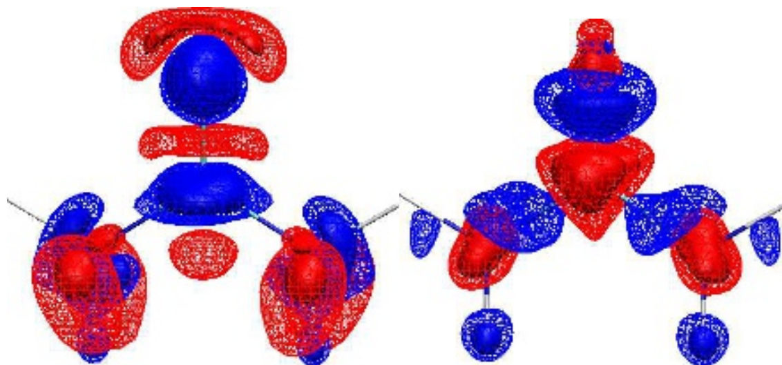
a) \lambda_{0.022,\text{BLYP}} - \lambda_{0.0,\text{BLYP}} , represents polarization ; N_e=0.32e b) \lambda_{0.046,\text{HF\_CC}} - \lambda_{0.0,\text{HF\_CC}} , represents correlation ; N_e=0.28e
