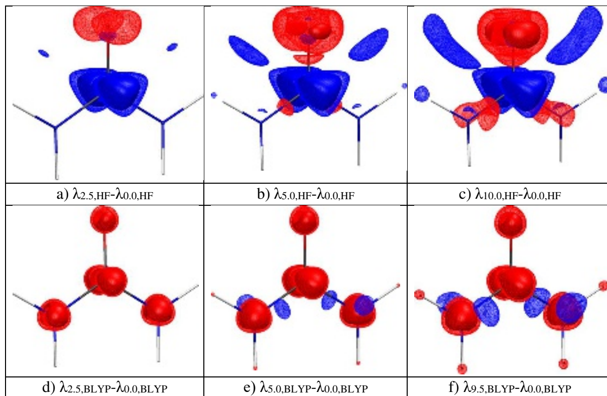
Figure 6. Plot of the difference in the exchange-correlation potential in form of the BLYP functional for different \lambda values during the XCW fitting of urea using CCSD structure factors of a maximum resolution of 1.4415 \text{ \AA}^{-1} . Individual details are given in subcaptions. Isosurface values in a.u. (solid/wireframe): +0.007/+0.005 (blue) and -0.007/-0.005 (red). Plots at the other two resolutions are given in the supplementary material.
