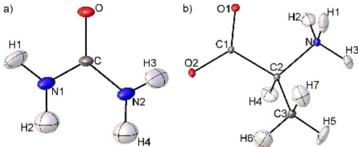
Figure 1. (a) HAR-refined structure of urea at RHF/pob-TZVP level of theory. Crystallographic details as of ref. 69 : space group = P\bar{4}2_1m (tetragonal), a = 5.5780(6) Å, b = 5.5780(6) Å, c = 4.6860(7) Å, V = 145.80(3) Å 3 . Measurement details as of ref. 69 : T = 123(2) K, \sin\theta_{\max}/\lambda = 1.4417 Å -1 . Refinement details from HAR: \text{Goof}^2 = 7.8748 , R = 0.0172 , wR = 0.0117 , min/max residual density = -0.101/0.079 eÅ -3 . (b) HAR-refined structure of L-alanine at RHF/pob-TZVP level of theory. Crystallographic details as of ref. 73 : space group = P2_12_12_1 (orthorhombic), a = 5.9279(10) Å, b = 12.2597(17) Å, c = 5.7939(9) Å, V = 421.1(1) Å 3 . Measurement details as of ref. 73 : T = 23(1) K, \sin\theta_{\max}/\lambda = 1.0778 Å -1 . Refinement details from HAR: \text{Goof}^2 = 1.5029 , R = 0.0198 , wR = 0.0169 , min/max residual density = -0.146/0.153 eÅ -3 . Anisotropic displacement parameters of all atoms are drawn at 50% probability level.
