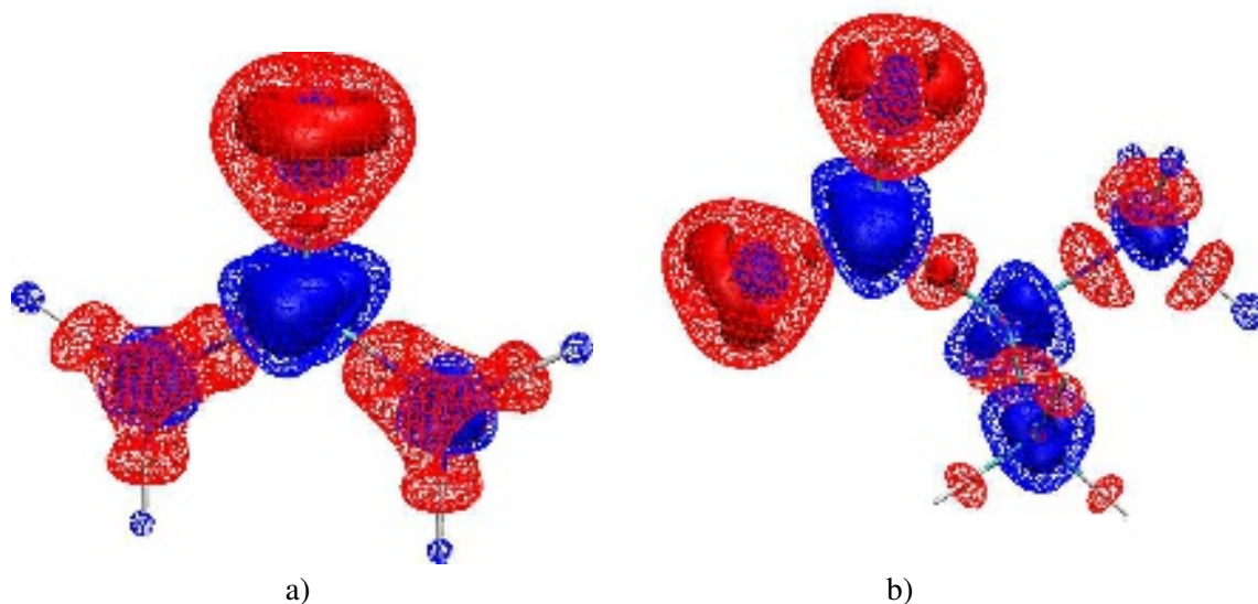
Figure 2. Plot of the difference between CCSD and HF electron densities used as reference for the reconstruction of electron correlation effects via XCW fitting for a) urea and b) L-alanine. Isosurface values in a.u. (solid/wireframe): +0.005/+0.0025 (blue) and -0.005/-0.0025 (red). 0.005 \text{ a.u.} = 0.005 e \text{ bohr}^{-3} = 0.034 e \text{ \AA}^{-3} . Total number of electrons shifted: 0.27 (urea), 0.40 (L-alanine).
