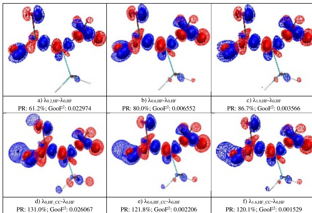
Figure 9. Plots of the difference in electron density for different \lambda values during the XCW fitting of L-alanine using structure factors from periodic-boundary calculations of a resolution below 1.0778 \text{ \AA}^{-1} . Individual details are given in subcaptions. Isosurface values in a.u. (solid/wireframe): +0.0025/+0.00125 (blue) and -0.0025/-0.00125 (red). Representations for the other resolutions are given in the supplementary material. CC = cluster charges.
