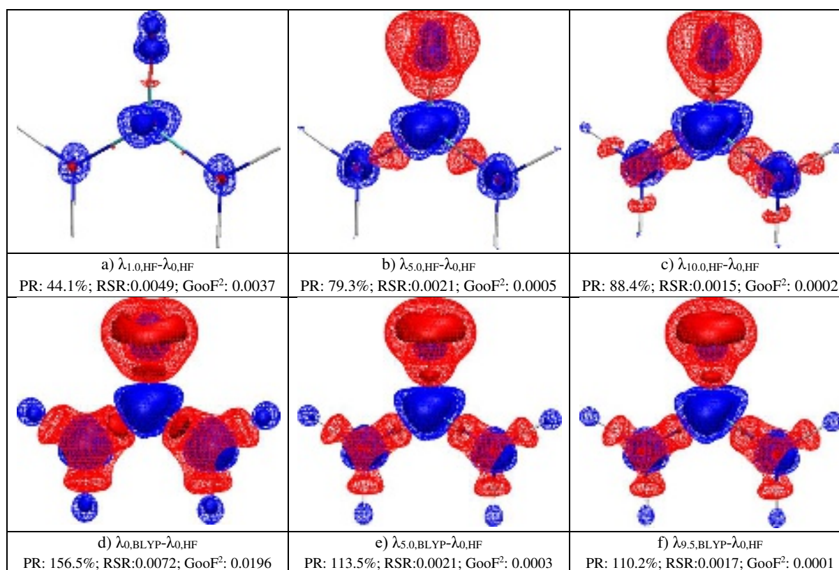
Figure 3. Plot of the difference in electron density for different \lambda values during the XCW fitting of urea using CCSD structure factors of a resolution below 1.4415 \text{ \AA}^{-1} . Individual details are given in subcaptions. Isosurface values in a.u. (solid/wireframe): +0.005/+0.0025 (blue) and -0.005/-0.0025 (red). Representations for the other resolutions are given in the supplementary material.
