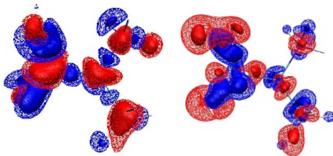
a) \lambda_{0.34,\text{BLYP}} - \lambda_{0.0,\text{BLYP}} , represents polarization ; N_e=0.52e b) \lambda_{0.53,\text{HF\_CC}} - \lambda_{0.0,\text{HF\_CC}} , represents correlation ; N_e=0.42e
