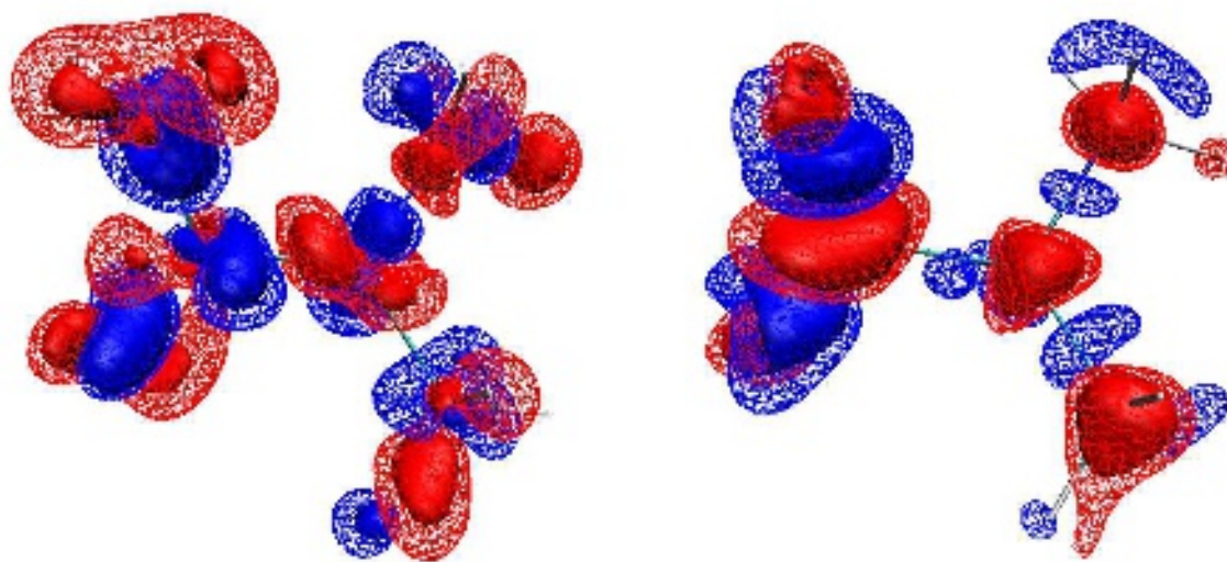
a) \lambda_{0.34,\text{BLYP}} - \lambda_{0.0,\text{BLYP}} , represents polarization ; N_e=0.52e b) \lambda_{0.53,\text{HF\_CC}} - \lambda_{0.0,\text{HF\_CC}} , represents correlation ; N_e=0.42e
