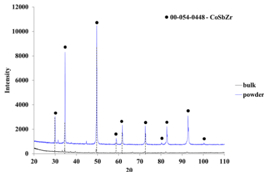
Figure 7: X-ray diffraction pattern of HH type-p bulk and final powder
