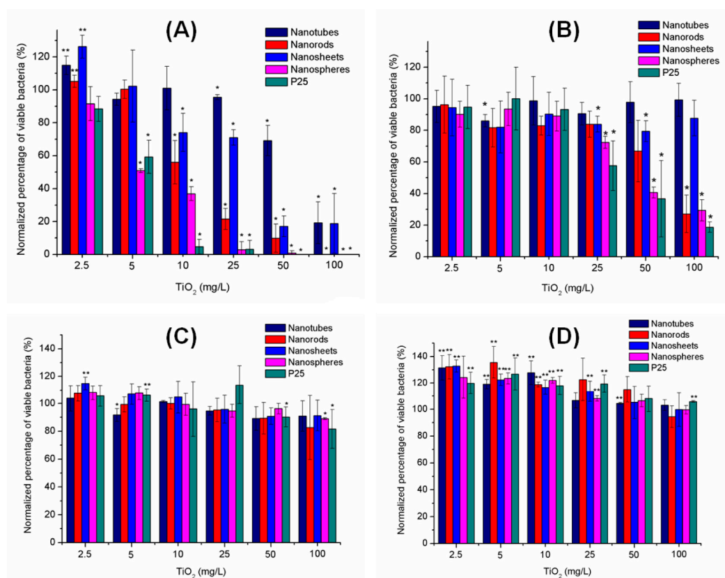
Figure 5. Bacterial viability of E. coli and A. hydrophila exposed to different \text{TiO}_2 -NPs. (A,B) E. coli (A) and A. hydrophila (B) under simulated solar irradiation. The exposure durations for E. coli and A. hydrophila were 1 h and 20 min, respectively. (C,D) E. coli (C) and A. hydrophila (D) in the dark for 1 h. One asterisk (*) indicates a statistically significant decrease in bacterial viability ( p < 0.05 ) compared to the \text{TiO}_2 -free control, whereas two asterisks (**) indicate an increase in bacterial viability ( p < 0.05 ). Reprinted with permission from [61] Copyright 2013 American Chemical Society.
