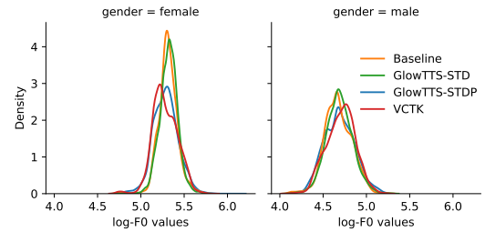
Figure 3: Log-F0 distribution of utterances generated with GlowTTS, GlowTTS-STD, GlowTTS-STDP, and the real VCTK utterances for both male and female speakers. Outliers due to F0 estimation errors have been removed.
