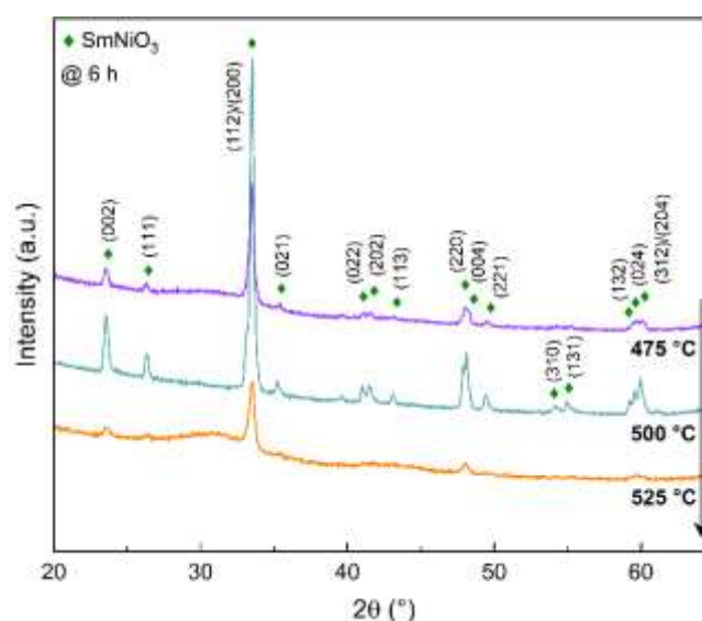
Figure 2. Comparison of the X-ray diffractograms after the in situ analysis for 6 h at 475 °C, 500 °C and 525 °C. The (hkl) labels correspond to the SmNiO 3 diffraction pattern (PDF n° 80-1948)
