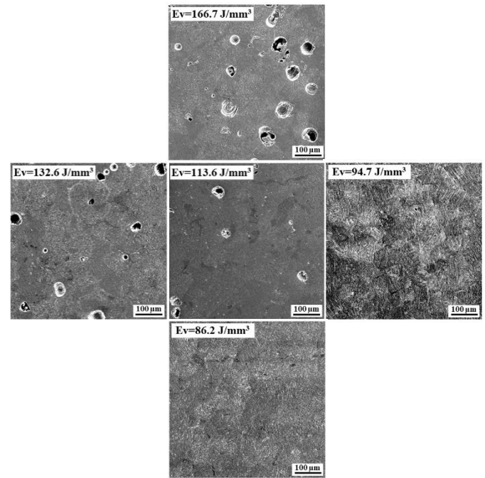
Fig 1. SEM observations of the 3d printing samples with the configuration of AM process parameters shown in Table 2.
