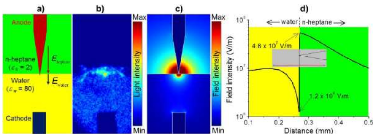
Fig. 10 a) Schematic of the experimental setup (not drawn to scale) showing the anode, the cathode, n-heptane, water, and the interface. b) ICCD image (integrated over 1 \mu s) of the discharge at the interface n-heptane-water (15 kV of applied voltage and 2 mm of gap distance). c) 2D electric field simulation using Comsol Multiphysics for conditions similar to b). d) Electric field profile along a line (the red line in the inset) crossing the interface close to the anode. After Hamdan et al. (2018) J Phys D: Appl Phys 51:244003. Reproduced with permission from the Institute of Physics.
