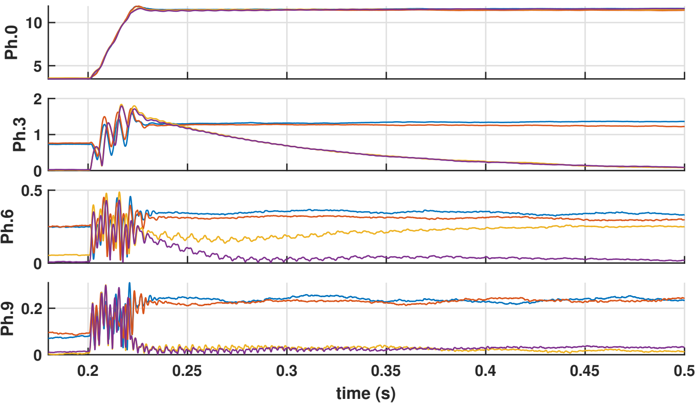
Moduli of Phasors
