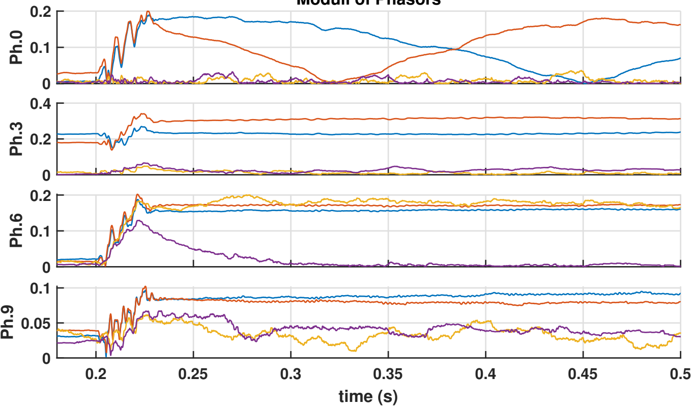
Moduli of Phasors
