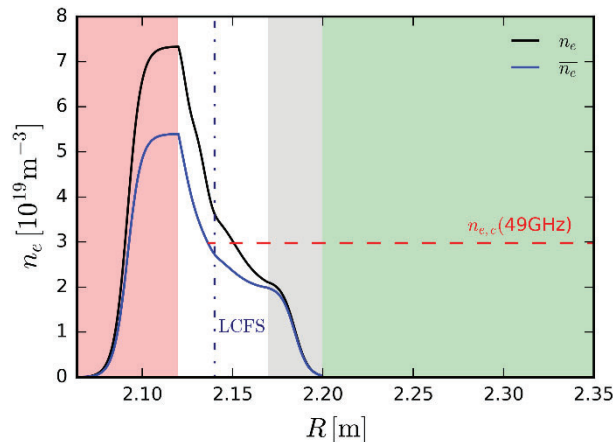
FIGURE 2. Radial electron density profiles from JOREK post-processed data used in REFNUM simulations. Profiles based on the fully perturbed data (black curve) and averaged data (blue curve) are shown. Color-shaded areas indicate different regions for: vacuum (green), modified hyperbolic tangent SOL transition (gray), JOREK data (white) and PML transition (red). The critical density layer for the probing frequency f_0 = 49 GHz is also displayed.
