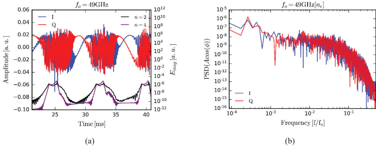
FIGURE 3. Time evolution of synthetic I(t) and Q(t) reflectometry signals using fixed frequency probing at f_o = 49\text{GHz} along a ELM cycle obtained from JOREK simulations, where the magnetic energy of the n = 2 and n = 4 modes are also displayed (a). Spectra of the corresponding reflectometry signals with the frequency axis normalized to the sampling frequency f_s (b).
