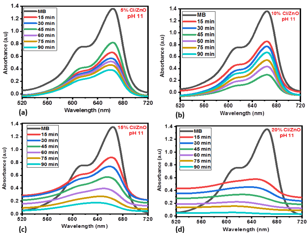
Figure 8 (a-d) UV-Vis absorbance spectra monitoring the concentration of MB after 15 min intervals of time for 5%, 10%, 15% and 20% Cl-doped ZnO at pH 11, respectively.
