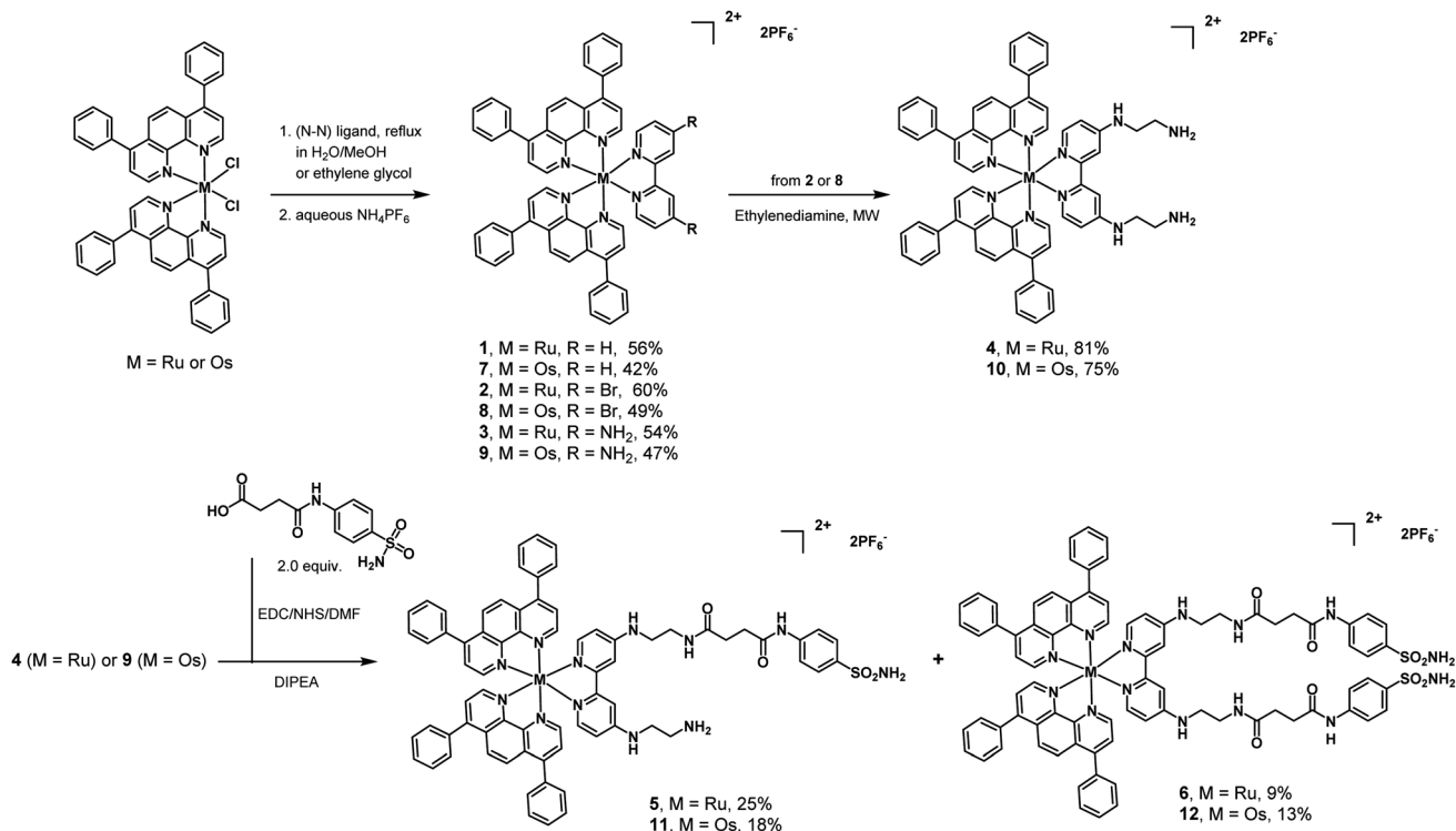
Scheme 1 Synthetic route and molecular structures of the complexes studied in this work. All complexes were isolated as PF 6 - salts. Biological experiments of the complexes were performed with the chloride counter-anion.
