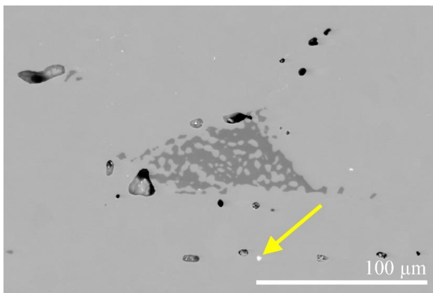
Fig. 2. SEM-BSE image of the \text{CeFe}_9\text{Si}_4 material. The matrix is the \text{CeFe}_9\text{Si}_4 phase, the darker-grey precipitates are the \text{Fe}_3\text{Si} phase and the white “spots” (one marked by an arrow) are the \text{CeFe}_2\text{Si}_2 phase. Some porosity is also visible.
