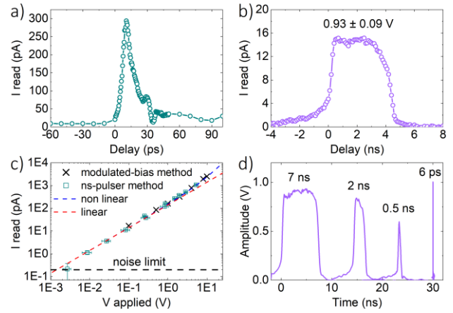
Fig. 2. a) A typical picosecond current pulse and b) 4 ns current pulse sampled by detector 1. c) The measured current as a function of the applied voltage to the detector, either statically (modulated bias method) or as pulses (nanosecond-pulsar method). Both methods give the same linear response. d) A few examples of pulses of variable amplitude detected by detector 1 ranging from 7 ns to 6 ps.
