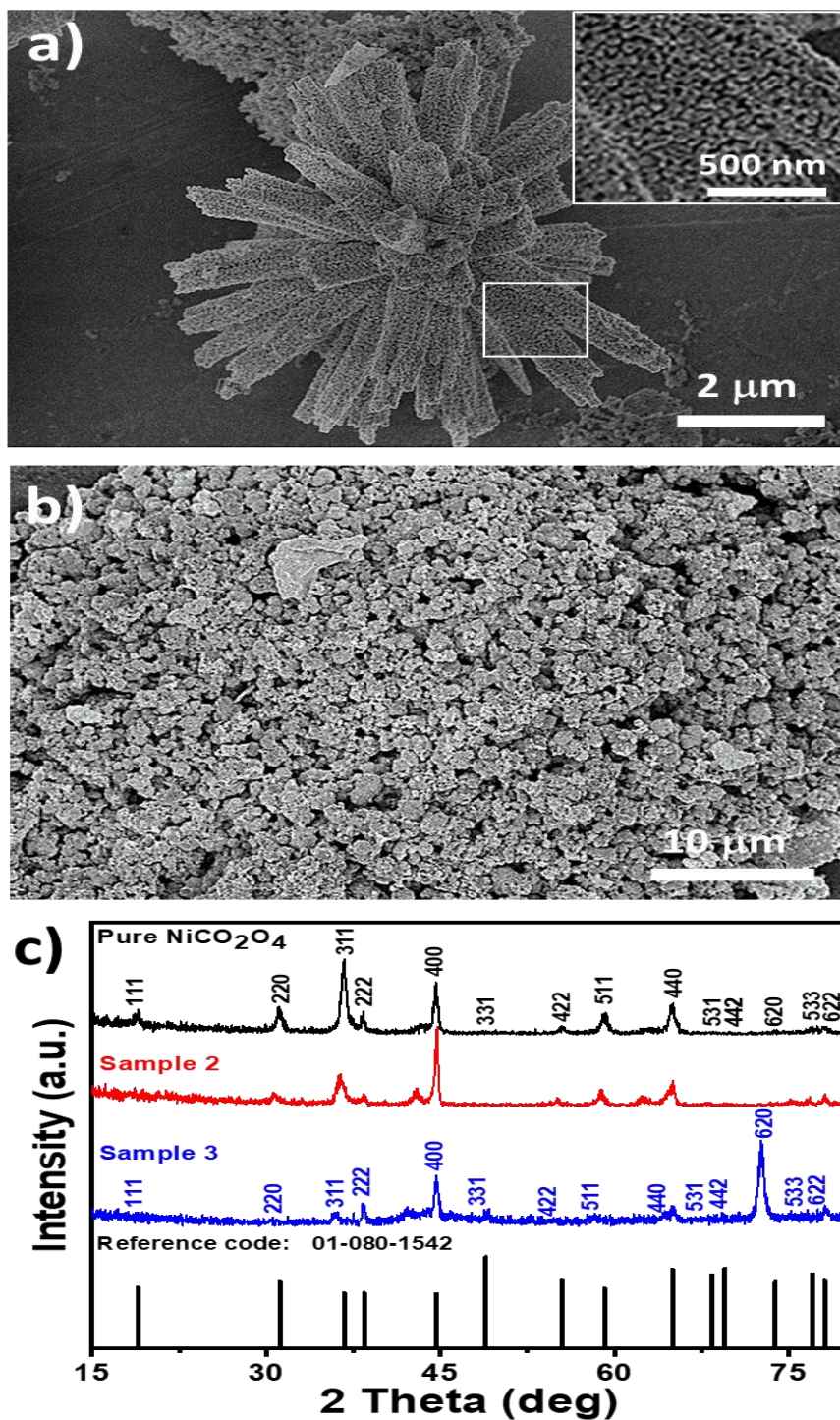
Figure 1: Distinctive SEM images at different magnifications of (a) pristine NiCo 2 O 4 nanostructures, (b) NiCo 2 O 4 nanostructures prepared with 1 mL (sample 2) and (c) XRD patterns of pristine NiCo 2 O 4 nanostructures, (b, c) NiCo 2 O 4 nanostructures prepared with 1 mL (sample 2), and 2 mL of lemon juice (sample 3).
