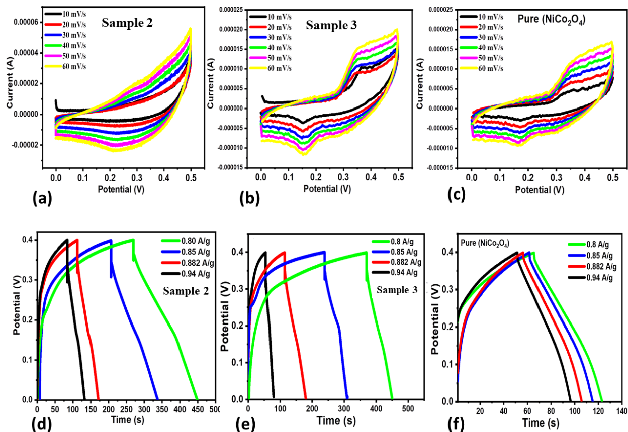
Figure 3: (a-c) Various CV curves at different scan rates for \text{NiCo}_2\text{O}_4 (sample 2), \text{NiCo}_2\text{O}_4 (sample 3), pure \text{NiCo}_2\text{O}_4 nanostructure, in 3.0M KOH aqueous electrolytic solution. (d-f)
