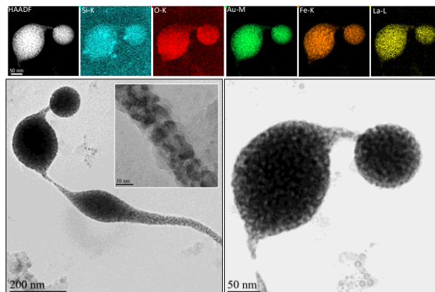
Fig. 4. Top: HAADF image and EDX elemental maps of elongated particles connected by 1D-assembly of particles of \sim 6\text{-}9 nm. Bottom left: larger view of the whole object. Insert: High-resolution image of 1D connection. Bottom right: TEM image showing the porous structure of the assembled particles.
