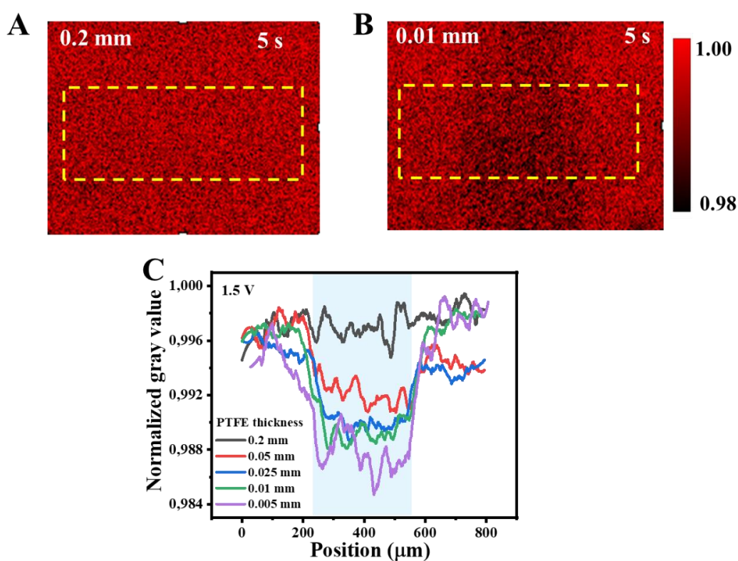
Fig. 5. The normalized gray value images of Au-IDE WE vs. WO_3 /ITO CE system at 1.5 V for 5 s, with WE-CE distance at 0.2 (A) and 0.01 mm (B); The average normalized gray value of the strips across the regions in the yellow dotted frames with different thickness of the PTFE spacer.
