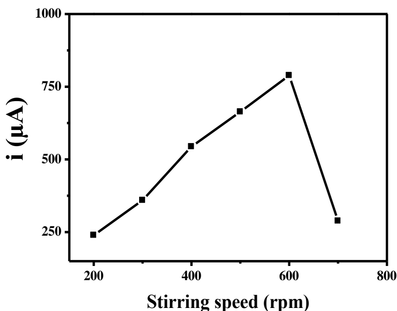
Fig. 10. Effect of mechanical stirring speed on peak current intensity by DPASV. [Hg 2+ ] 35 µmol.L -1 ; scan rate 20 mV/s; deposition time 120 s; pulse amplitude 50 Mv
