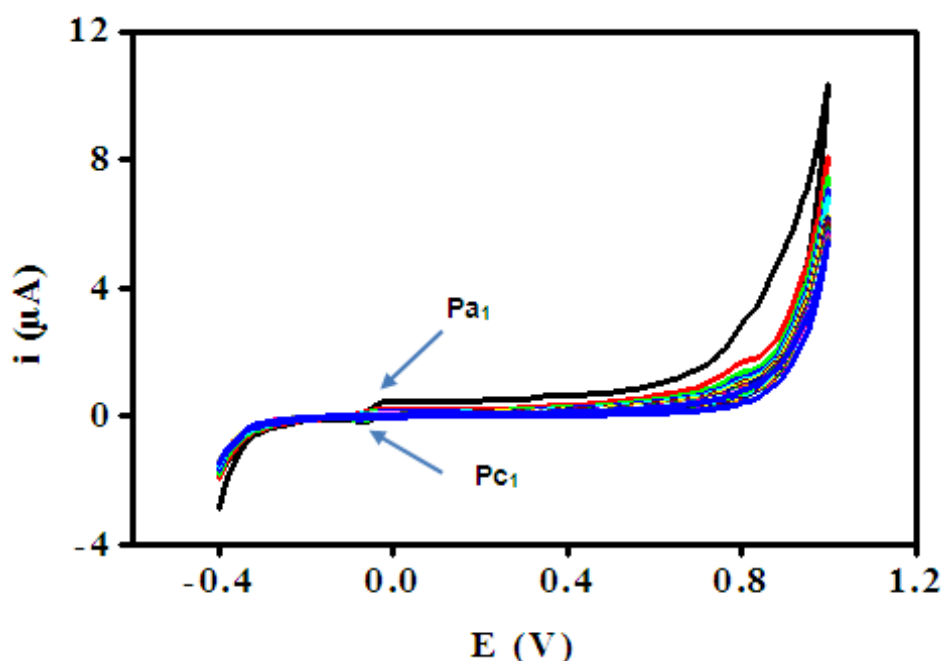
Fig. 1. Cyclic voltammograms recorded for the polymerization of Eriochrome blue black R at the carbon paste electrode in 0.1 \text{ mol.L}^{-1} of \text{NaOH} containing 300 \mu\text{mol.L}^{-1} of monomer during 25 cycles. Scan rate, 100 \text{ mV.s}^{-1}
