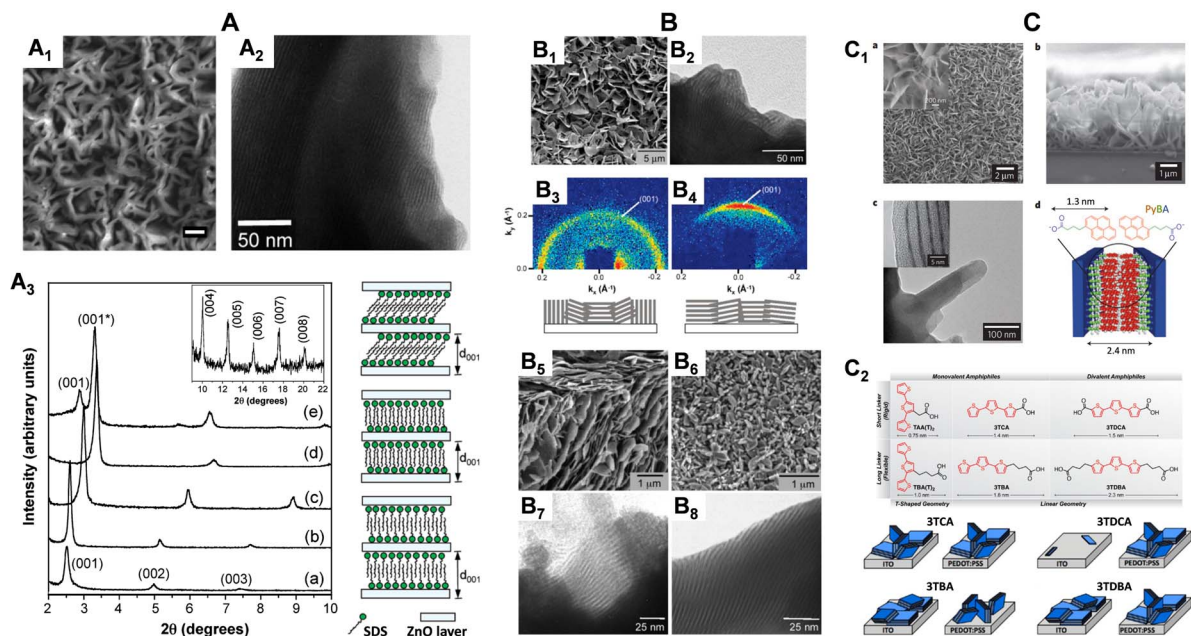
Figure 20. (A) Cathodically electrodeposited ZnO films. (A 1 ) SEM image (scale bar: 1 \mu\text{m} ) and (A 2 ) TEM view of lamellar-structured ZnO films deposited (at -0.5 V for 10 min at 70 ^{\circ}\text{C} ) from 0.02 M \text{Zn}(\text{NO}_3)_2 solutions containing either 0.25 wt% of SDS (A 1 ) or 0.25 wt% of AOT (A 2 ) anionic surfactants. (A 3 ) Small-angle XRD patterns of ZnO films deposited from 0.02 M \text{Zn}(\text{NO}_3)_2 solutions containing (a) 0.02 wt% of SHDS, (b) 0.02 wt% of SDBS, (c) 0.25 wt% of DP, (d) 0.25 wt% of AOT, and (e) 0.25 wt% of SDS, with possible variation of SDS lamellar assemblies that can lead to different repeat distances on the right. Reprinted from Tan et al. [235], Copyright (2005) American Chemical Society. (B) Anodically electrodeposited ZnO films. (B 1 ) SEM image and (B 2 ) TEM view of lamellar-structured ZnO films deposited (at +0.15 V for 30 min at 65 ^{\circ}\text{C} ) from solutions containing 0.02 M ascorbic acid and 0.01 M \text{Zn}(\text{NO}_3)_2 (at a pH of 13.3) and 5 wt% of lauric acid surfactant. (B 3 , B 4 ) 2D gi-SAXS of ZnO films deposited (B 3 ) with 10 wt% of SDS and (B 4 ) with 5 wt% of lauric acid. (B 5 –B 8 ) SEM (B 5 , B 6 ) and TEM (B 7 , B 8 ) images of ZnO films templated by (B 5 , B 7 ) 5 wt% of SDS and 1 wt% of CTAB or (B 6 , B 8 ) 5 wt% of SDS and 1 wt% of TAB. Reprinted from Steinmiller and Choi [236], Copyright (2007) American Chemical Society. (C) Lamellar hybrid nanostructures electrodeposited with the aid of conjugated surfactant molecules. (C 1 ) Morphology: (a, b) SEM images (top (a) and cross-sectional (b) views) of deposited ZnO platelets using PyBA (magnified in the inset for image (a)); (c) TEM image of lamellar sheets within platelets, magnified in the inset; (d) schematic diagram of lamellar ordering composed of inorganic Zn-rich regions and bilayers of PyBA surfactant. Reproduced with permission from Sofos et al. [454], Copyright (2009) Nature Publishing Group. (C 2 ) Structures of the terthiophene-based surfactants (with systematic modifications of their geometry, valency, and flexibility) used for the cathodic electrodeposition of lamellar ZnO films on ITO and PEDOT:PSS-coated electrodes: TAA(T) 2 and TBA(T) 2 do not lead to ZnO film growth, 3TCA grows isotropic lamellae on both substrates, lamellar coverage from 3TDCA deposition are too weak for a 2D gi-SAXS signal on ITO and isotropic on PEDOT:PSS, 3TBA directs parallel growth on ITO and perpendicular growth on PEDOT:PSS, and 3TDBA deposits lamellae that are preferentially parallel on ITO and isotropic on PEDOT:PSS. Reprinted from Bruns et al. [455], Copyright (2013) American Chemical Society.
