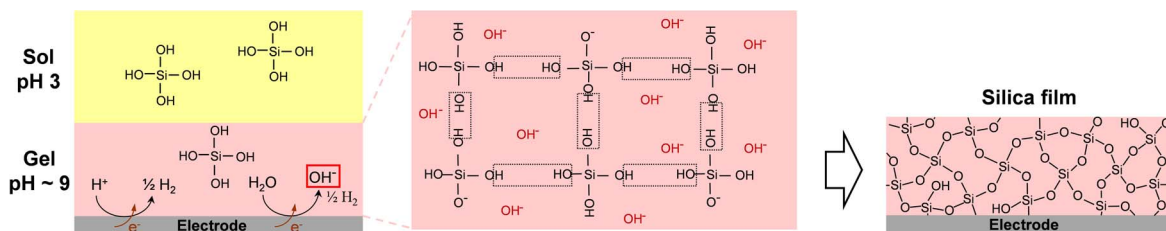
Figure 1. Schematic illustration of the electro-assisted deposition of a silica film onto an electrode surface from a hydrolysed sol at pH 3 (yellow part) by applying a cathodic potential likely to increase pH at the electrode/solution interface (pink part) to induce gelation of the sol and formation of the silica network by condensation of \text{Si}(\text{OH})_4 precursors catalysed by the electrogenerated \text{OH}^- species.
