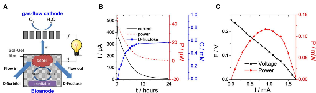
Figure 8. (A) Illustration of the flow bioreactor composed of a gas-flow cathode and a bioanode made of carbon felt (16 cm 2 ) modified with carbon nanotubes, wrapped with poly(methylene green) mediator, and subsequently subjected to electrodeposition of a biocomposite layer from a sol solution containing TEOS, GPS, PEI and DSDH (the enzyme concentration in the bioanode was 0.375 mg·cm -3 ). (B) Conversion of D-sorbitol (1 mM initial concentration) to D-Fructose in the bioreactor with simultaneous energy production. The 100 mL flowing electrolyte was composed of 0.1 M Tris-HCl buffer (pH 9) and 0.1 mM NAD + . (C) Polarization curve of the bioreactor when flowing the D-sorbitol solution. Reprinted from Mazurenko et al. [275], Copyright (2016), with permission from Elsevier Science.
