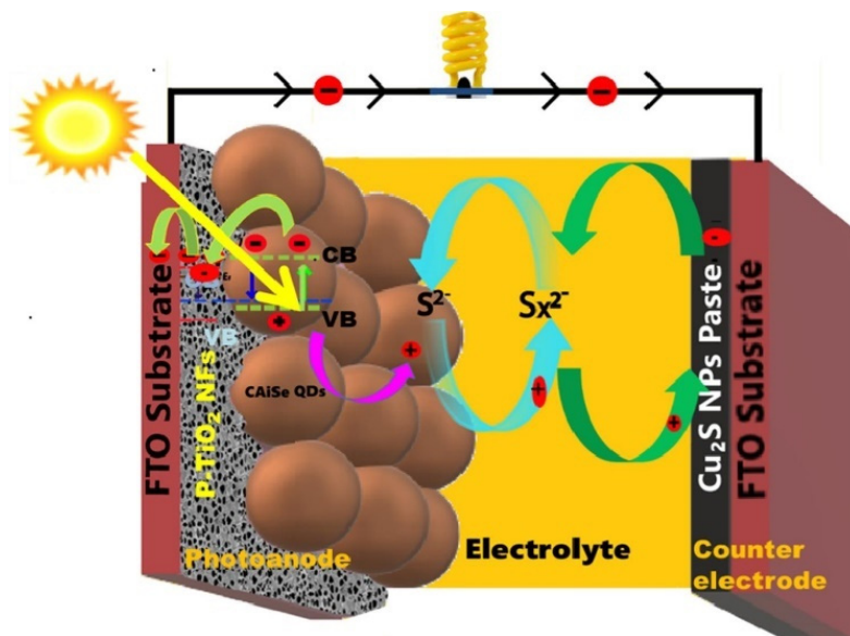
Figure 15. Schematic representation of the fabricated QDSSC. Used with permission from ref. [82]. Copyright 2020 Elsevier.
