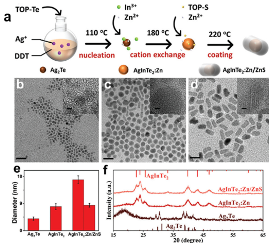
Figure 5. (a) Scheme for the synthesis of \text{AgInTe}_2\text{:Zn/ZnS} NCs. TEM images of the as-synthesized (b) \text{Ag}_2\text{Te} , (c) \text{AgInTe}_2\text{:Zn} , and (d) \text{AgInTe}_2\text{:Zn/ZnS} NCs (Scale bar = 20 nm). Insets show their corresponding high-resolution TEM images (Scale bar = 2 nm). (e) Size distribution histograms of the as-synthesized NCs through calculating 200 nanoparticles in their TEM images. (f) Powder XRD patterns of the as-synthesized \text{Ag}_2\text{Te} , \text{AgInTe}_2\text{:Zn} and \text{AgInTe}_2\text{:Zn/ZnS} NCs, respectively. Used with permission from ref. [44]. Copyright 2022 RSC publishing.
