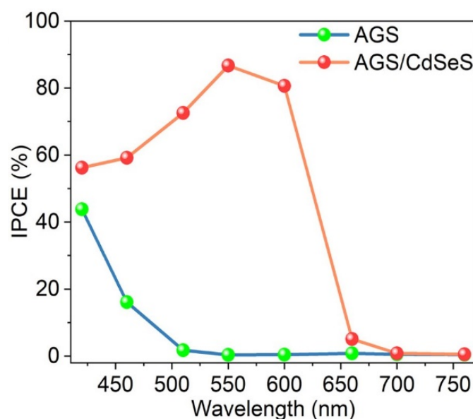
Figure 12. IPCE spectra of AGS core and AGS/CdSeS core/shell QDs-based PEC cells. Used with permission from ref. [68]. Copyright 2021 Elsevier.
