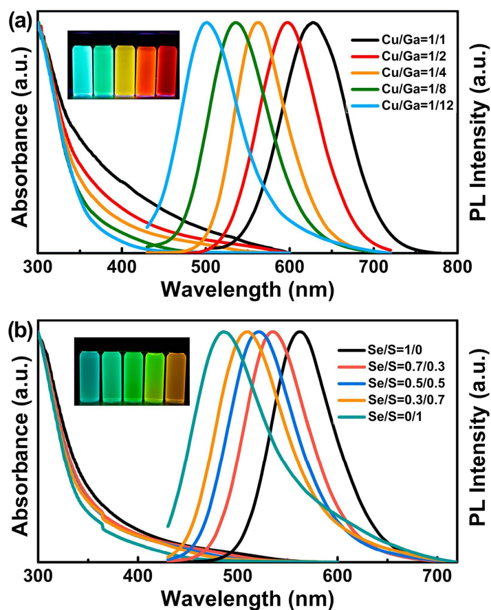
Figure 17. UV-vis absorption (left) and PL spectra (right, \lambda_{\text{ex}} = 405 nm) of (a) CGSe/ZnSe and (b) CGSe x S 1-x /ZnSeS QDs prepared under various Cu/Ga and Se/S precursor molar ratios, respectively. Inset: digital photograph of samples under the radiation of a 365 nm UV lamp. Used with permission from ref. [90]. Copyright 2018 Elsevier.
