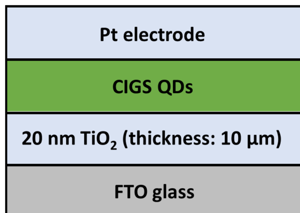
Figure 8. Sandwich-type CIGS-based QDSSC (Adapted from ref. [53]).
