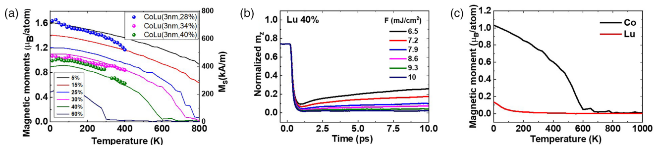
FIG. 5. (a) Magnetic moment versus temperature for \text{Co}_{1-x}\text{Lu}_x alloys with various lutetium concentrations, x . Dots indicate experiments; lines indicate simulations. (b) Simulations of the cobalt demagnetization dynamics for the \text{Co}_{60}\text{Lu}_{40} alloy as a function of laser power. (c) Simulations of the magnetic moment versus temperature for both cobalt and lutetium subnetworks in case of \text{Co}_{60}\text{Lu}_{40} .
