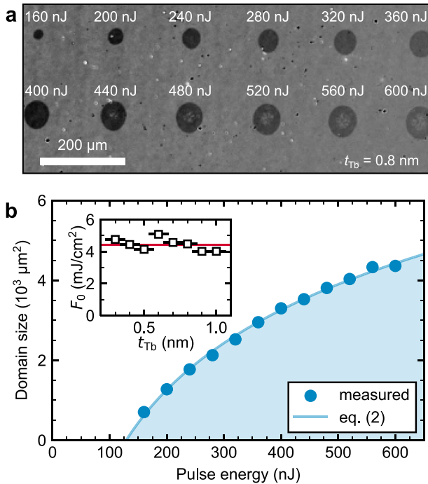
FIG. 3. (a) Kerr microscopy images of the Tb(0.8 nm)/Co/Gd(1 nm)/Co/Tb(0.8 nm) sample after excitation by a single fs linearly polarized laser pulses with energies indicated in the Figure. (b) Sizes of reversed domains as a function of laser pulse energy extracted from (a). The continuous line is a best fit according to Eq. (2). The inset shows the critical fluence for AOS as a function of Tb thickness with the horizontal red line indicating the mean value of 4.44 mJ/cm 2 .
