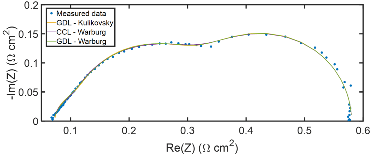
Figure 4. Experimental Nyquist diagram measured in operando (0.5 A cm -2 and 0.68 V, under H 2 /air) with cell A1 in the operation conditions described in section 2.3 and fitting curves obtained with the different EECs depicted in Figure 2 [39].
