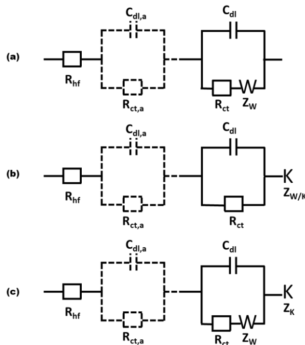
Figure 2. EECs used in this work: the membrane and cathode (solid lines) are modeled either by (a) a usual Randles circuit with the diffusion impedance (Warburg) inside the CCL circuit implying oxygen transport limited by the CCL (pores or ionomer layer), or (b) a modified Randles circuit with the diffusion impedance (Warburg or Kulikovsky) in series with the CCL circuit implying the GDL limiting for O_2 diffusion. Circuit (c) accounts for both oxygen diffusion impedances, the CCL and GDL. The anode is optionally taken into account through a parallel connection of a charge transfer resistance R_{ct,a} and a double-layer capacitance C_{dl,a} (dotted lines).
