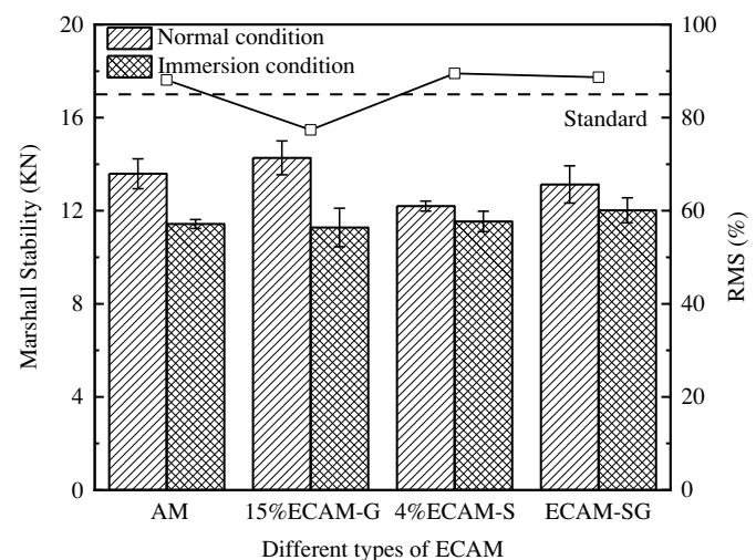
Fig. 14. Marshall stability and RMS of ECAMs.
