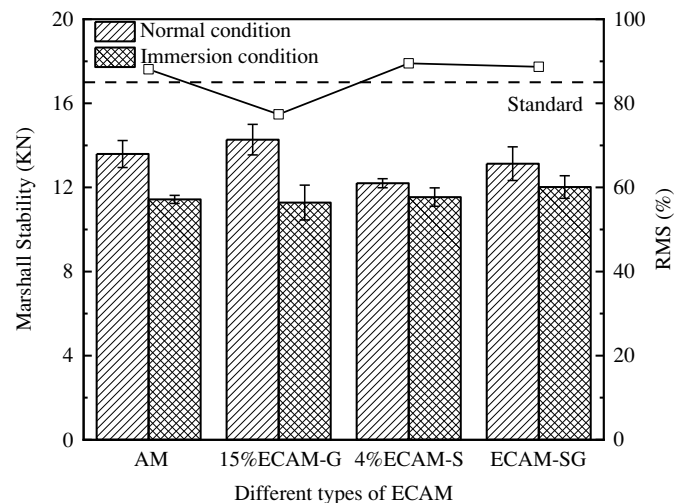
Fig. 14. Marshall stability and RMS of ECAMs.
