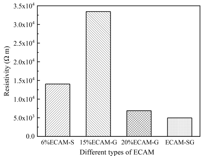
Fig. 13. Electrical resistivity values of different ECAMs.
