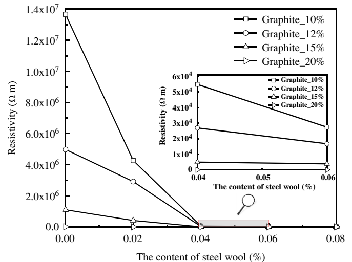
Fig. 11. Resistivity values of ECAM-SG.
